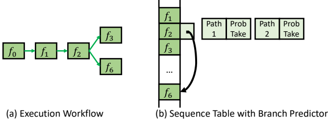
Fig. 8: Example of execution workflow (a) and corresponding Sequence table with Branch Predictor (b).
