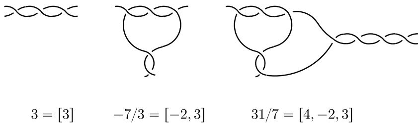
Figure 5. Examples of rational tangles.
