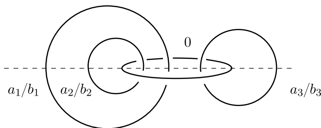
Figure 3. The manifold Y(a_1/b_1, a_2/b_2, a_3/b_3) .
