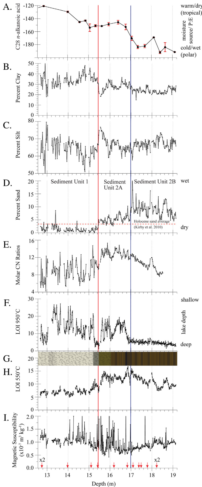
Fig. 4. Sedimentological and geochemical data for LEDC10-1 with stratigraphic column. A) \delta D_{wax} (‰) ( C_{28} n-alkanoic acid), B) Percent clay, C) Percent silt, D) Percent sand, E) Molar C:N ratios, F) LOI 950 °C (Percent (%) total carbonate), G) Stratigraphic column, H) LOI 550 °C (Percent (%) total organic matter), I) Magnetic susceptibility. Red arrows represent age control. Vertical red and blue lines represent the statistically defined sediment unit boundaries based on Figs. 5 and 6 (see Discussion).
