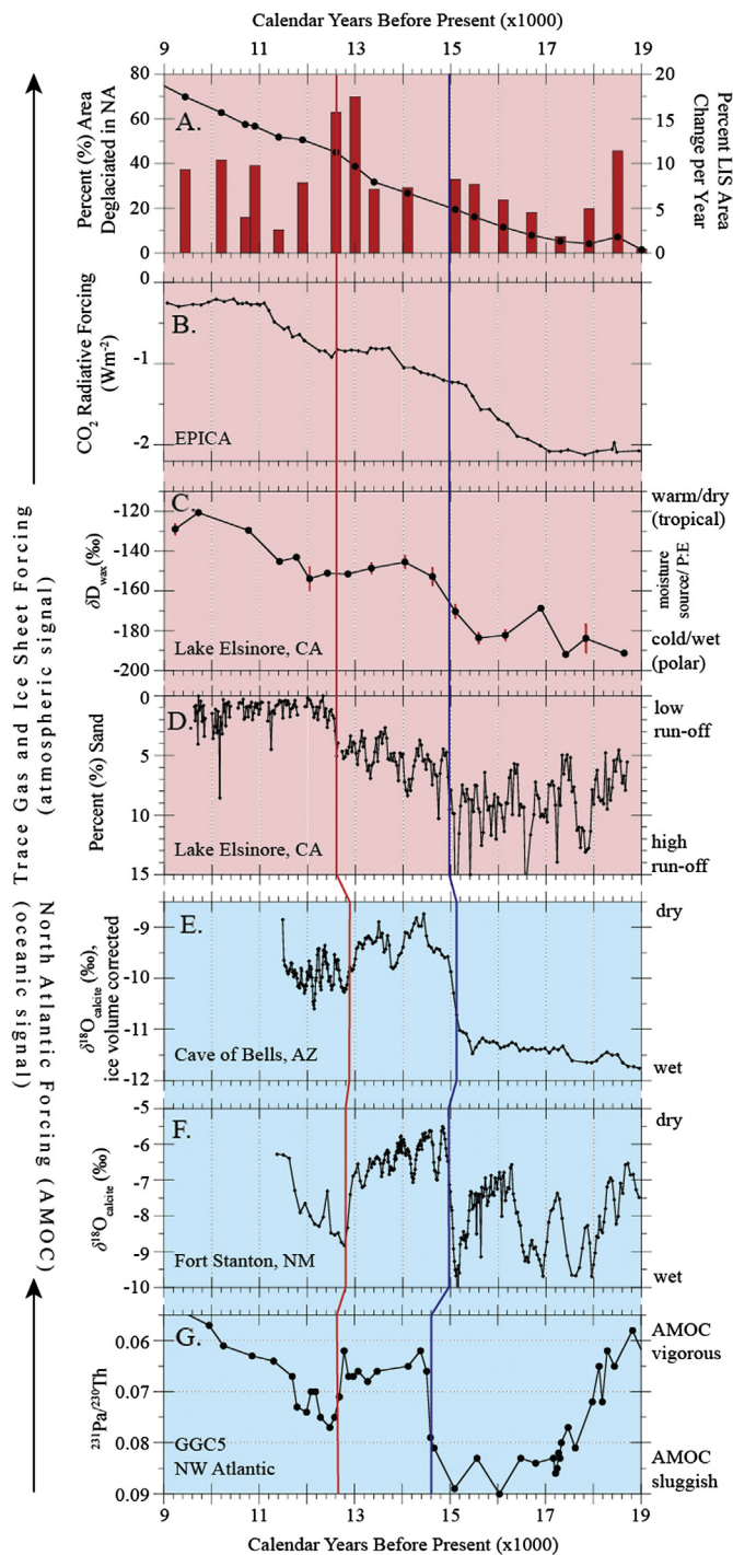
Fig. 9. Regional deglacial sequences and forcings. A) Left Y-axis (black dotted line): Percent (%) area deglacialated in North America per year (Dyke, 2004), Right Y-axis: Percent (%) Laurentide Ice Sheet (LIS) area change per year (Dyke, 2004), B) CO_2 radiative forcing ( Wm^{-2} ) per year (Joos and Spahni, 2008), C) \delta D_{wax} (‰) ( C_{28} n -alkanoic acid), D) LEDC10-1 percent (%) sand, E) Cave of Bells oxygen isotope data (Wagner et al., 2010), F) Fort Stanton oxygen isotope data (Asmerom et al., 2010), G) ^{231}Pa/^{230}Th data (McManus et al., 2004). See text for data details. NA = North America.
