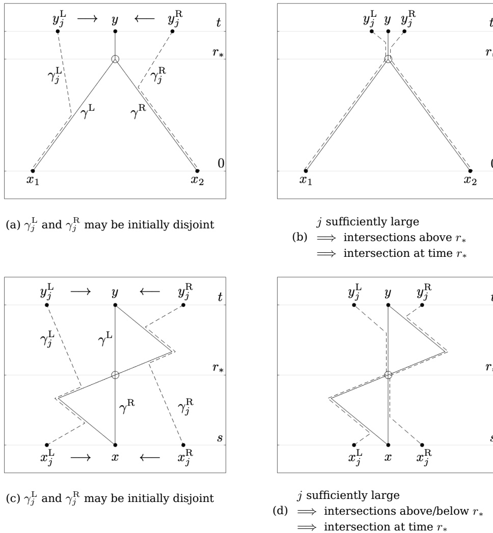
Figure 9: Geodesics considered in the proof of Proposition 4.1. Diagrams (a) and (b) illustrate the argument for \text{Supp}(\mu_{x_1, x_2; t}) \subset \mathcal{D}_{x_1, x_2; t} , while (c) and (d) illustrate the argument for \text{Supp}(\mu_{s; t}) \subset \mathcal{D}_{s; t} . In each case, there is assumed to be some intermediate time r_* at which \gamma^L and \gamma^R intersect; the point of intersection is marked with an open circle. If \gamma_j^L intersects \gamma^L in (a), then the two geodesics coincide at all lower times; similarly for \gamma_j^R with \gamma^R . When j \rightarrow \infty , both pairs must experience intersections above time r_* , thereby forcing an intersection between \gamma_j^L and \gamma_j^R at time r_* , where \gamma^L and \gamma^R agree. A slightly different argument is needed for the scenario in (c). If \gamma_j^L intersects \gamma^L at two distinct times, then the two geodesics coincide at all times in between; similarly for \gamma_j^R with \gamma^R . For both pairs, sending j \rightarrow \infty forces at least one intersection before time r_* and one after time r_* . Hence a common intersection eventually appears at r_* .
