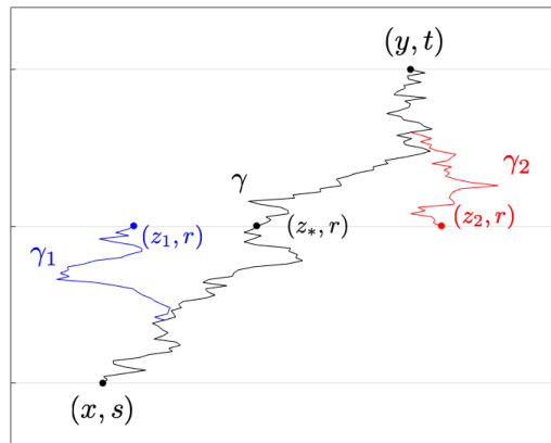
Figure 3: Example geodesics in \mathcal{L} . Time is visualized in the vertical direction. Shown above is a geodesic \gamma between (x, s) and (y, t) that passes through (z_*, r) , meaning z_* achieves the supremum in (1.9). For generic z_1 \neq z_* , geodesics \gamma_1 and \gamma will typically coincide for some random length of time, and then remain disjoint after said time. Similarly, geodesics \gamma_2 and \gamma will typically coincide for all times after their first intersection.
