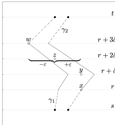
Figure 7: Scenario implied by \mathcal{B}_\varepsilon . Because s, t \in [-m, m] satisfy t - s \geq 6\delta , there is some r \in [-m, m] \cap 3\delta\mathbb{Z} for which [r, r + 3\delta] is a subinterval of [s, t] . This subinterval is divided into three further subintervals, each of which admits the two disjoint subgeodesics arising from \gamma_1 and \gamma_2 . (Here, three is the minimum number needed for our analysis to ensure probability 0, but it could be replaced by any larger integer.) The points x, y, z, w \in [-m, m] \cap \varepsilon\mathbb{Z} are chosen so that intervals of radius \varepsilon about these points contain both \gamma_1 and \gamma_2 at the associated times.
