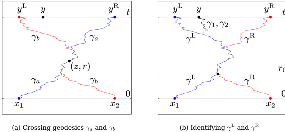
Figure 10: Geodesics considered in the proof of Proposition 4.1 for showing \mathcal{D}_{x_1, x_2; t} \subset \text{Supp}(\mu_{x_1, x_2; t}) . In (a), the geodesics \gamma_a : (x_1, 0) \rightarrow (y^R, t) and \gamma_b : (x_2, 0) \rightarrow (y^L, t) must intersect by planarity; the point (z, r) can be any intersection point. In (b), it is assumed that y \notin \text{Supp}(\mu_{x_1, x_2; t}) , which implies that the paths \gamma^L : (x_1, 0) \rightarrow (y^L, t) and \gamma^R : (x_2, 0) \rightarrow (y^R, t) , formed by concatenating the relevant portions of \gamma_a and \gamma_b , are geodesics. Any geodesic \gamma_1 : (x_1, 0) \rightarrow (y, t) cannot pass to the left of \gamma^L , while any geodesic \gamma_2 : (x_2, 0) \rightarrow (y, t) cannot pass to the right of \gamma^R . Shown here is the typical situation in which \gamma_1 and \gamma_2 initially coincide with \gamma^L and \gamma^R , respectively. Hence \gamma_1 and \gamma_2 will coalesce at the same time r_0 at which \gamma^L and \gamma^R first intersect, although in principle \gamma_1 and \gamma_2 may intersect earlier.
