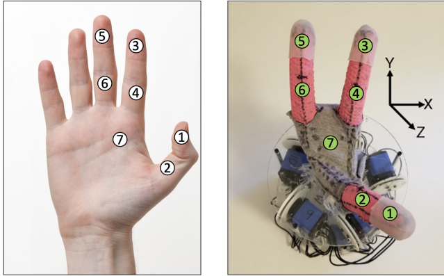
Fig. 4: One-to-One Mapping between Human Hand and Soft Robotic Hand. Position 7 represents the furthest point from the contact points.
