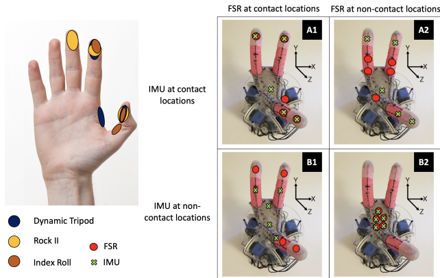
Fig. 5: Marked contact points on the human hand (left) and Selected Sensor Placement Configurations (right).
