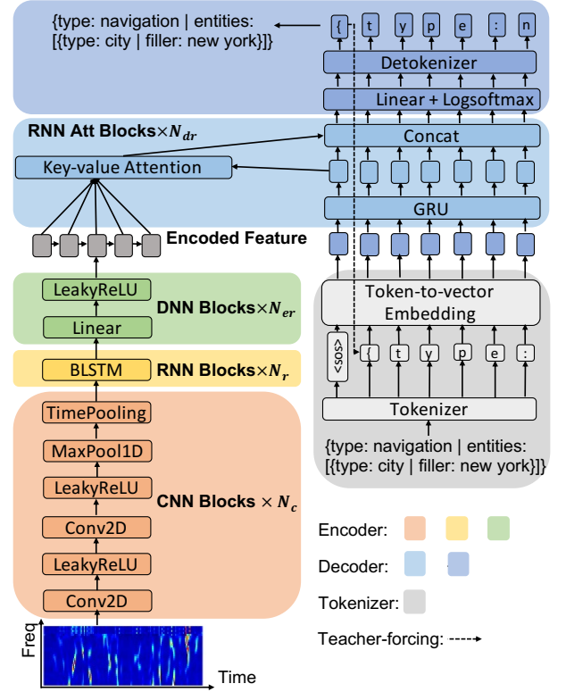
Figure 6. Model Architecture
