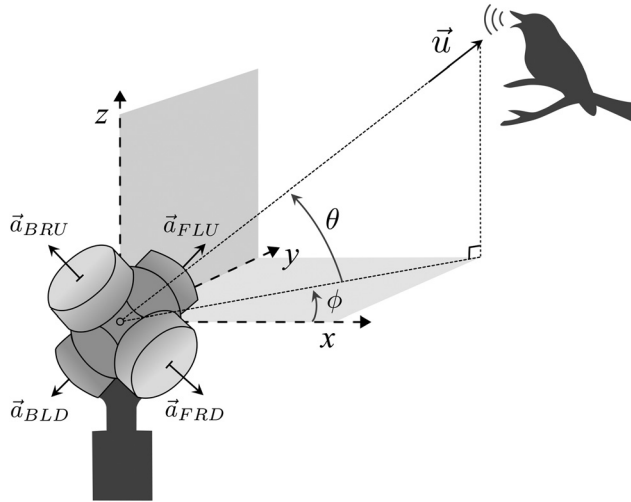
FIG. 1. A first-order ambisonic microphone, comprised of four co-located capsules, is one design for an AVS. The four cardioid capsules are oriented in a tetrahedron, with axes \vec{a}_{FLU}^T (front-left-up), \vec{a}_{FRD}^T (front-right-down), \vec{a}_{BLD}^T (back-left-down), and \vec{a}_{BRU}^T (back-right-up). The azimuth angle \phi and elevation angle \theta define the direction-of-arrival unit vector \vec{u} relative to the microphone.
