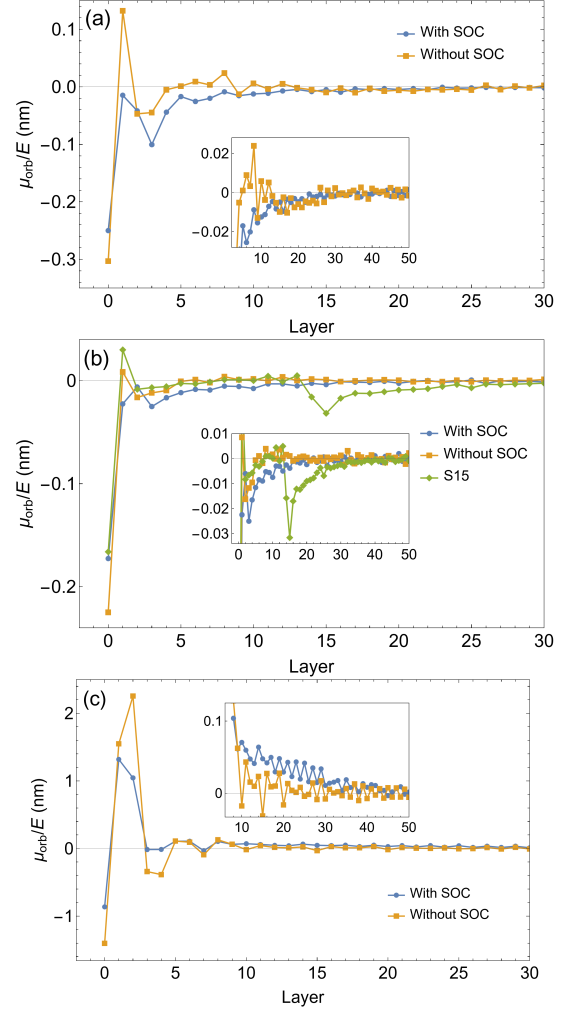
FIG. 5. Orbital accumulation profiles \mu_{\text{orb}}(z)/E in a 100-ML Pt film with (a) V_m = 40 mRy at E = E_F , (b) V_m = 80 mRy at E = E_F , and (c) V_m = 40 mRy at E = E' calculated with or without spin-orbit coupling (SOC). Panel (b) includes the data for the S15 system which has spin-orbit coupling turned off in 15 monolayers of Pt near each surface. Insets show the same data on smaller scales.
