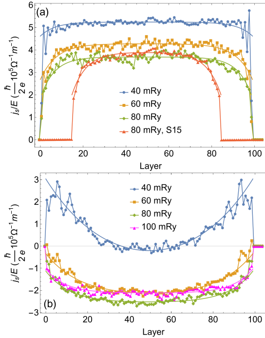
FIG. 3. Spin current in the Pt film expressed as shown in Eq. (12) in units of 10^5 \frac{\hbar}{2e} \Omega^{-1} m^{-1} . The calculated intrinsic spin-Hall conductivity of Pt reported in the literature is close to 4 \times 10^5 \frac{\hbar}{2e} \Omega^{-1} m^{-1} . The smooth lines are fits to Eq. (8) where l_{sf}^T is taken from the spin accumulation fits. (a) At E = E_F . (b) At E' = E_F - 2.72 eV.
