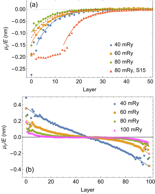
FIG. 2. Spin accumulation profile \mu_y(z)/E in a 100-ML film of Pt with Anderson disorder strengths shown in the legends, calculated at (a) the physical Fermi level, or (b) with the Fermi level shifted to -2.72 eV. Only part of the film is shown in panel (a). Solid lines are fits to Eq. (6). The red line marked S15 in panel (a) corresponds to the calculation with spin-orbit coupling turned off in 15 ML of Pt near each interface. The dashed red line is shifted to the left by 15 ML.
