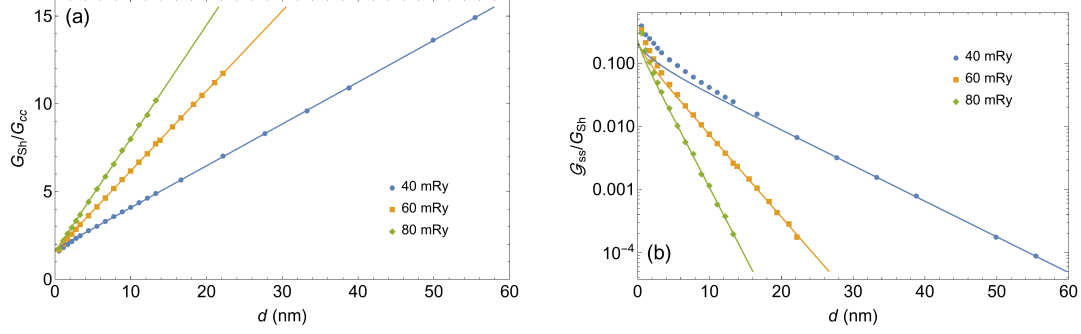
FIG. 7. Fits of the calculated (a) reduced resistance G_{SH}/G_{cc} and (b) the reduced spin conductance \mathcal{G}_{ss}/G_{SH} as a function of the layer thickness d in bulk Pt calculated at E_F using the 16 \times 1 lateral supercell.
