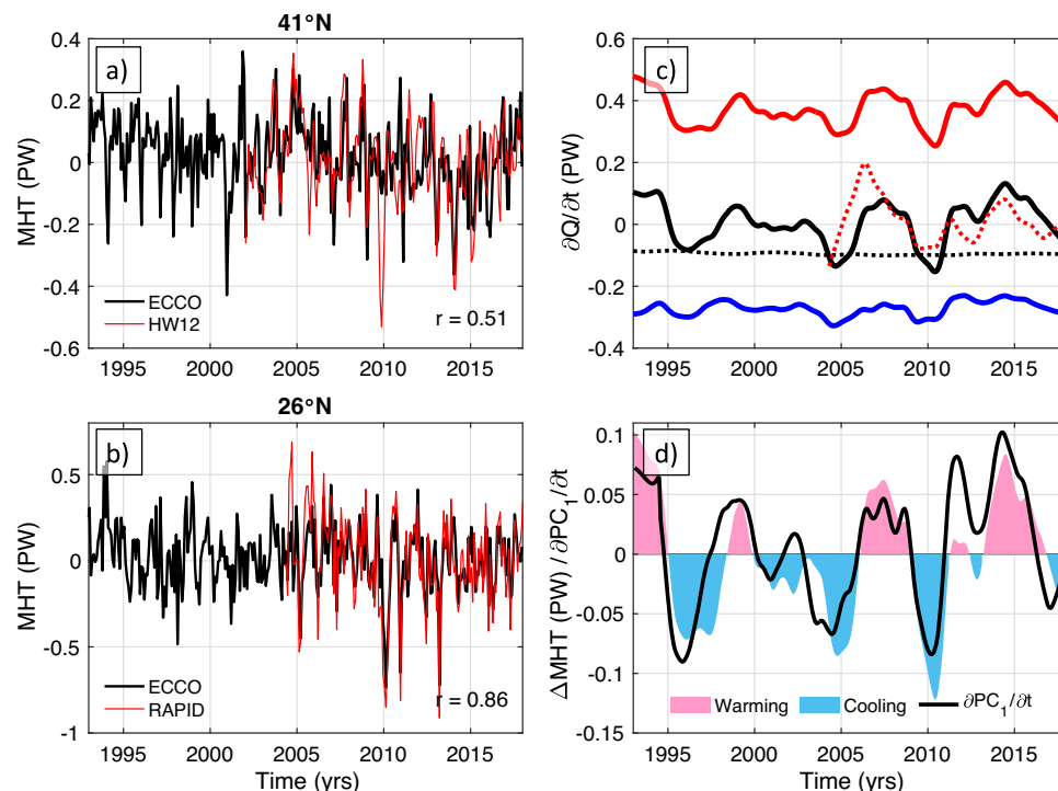
Fig. 2 | Oceanic heat budget in the subtropical North Atlantic. a The time series of the meridional heat transport anomalies relative to the common time intervals at 41^\circ\text{N} (black) in the ECCO model and (red) from Hobbs and Willis, 2012 (HW12); b the time series of the meridional heat transports (black) in the ECCO model at 26^\circ\text{N} and (red) from RAPID observations at about 26^\circ\text{N} ; c the full-depth ocean heat budget between 26^\circ\text{N} and 41^\circ\text{N} : (black) the time-change in Oceanic Heat Content, (red) heat advection, (blue) the volume-weighted averaged forcing term that includes surface forcing, penetrated shortwave radiation, and geothermal forcing,
