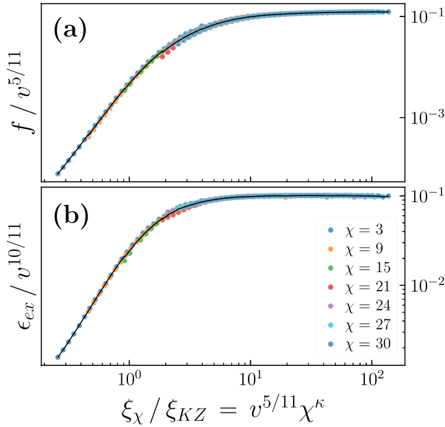
FIG. 3. The scaling function collapse for the fidelity density and excitation energy in the three-state Potts model. The length scale introduced by the bond dimension, \xi_\chi is a power law with exponent given by Eq. (11), with a central charge of c = 4/5 .
