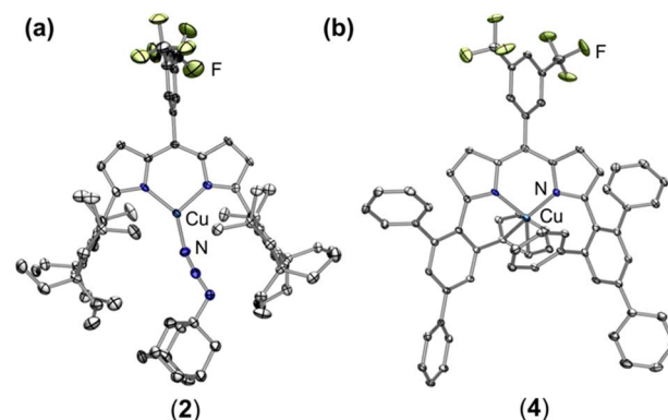
Fig. 3 Solid state molecular structures of (a) (EMindL)Cu(N 3 Ad) ( 2 ) and (b) (ArFL)Cu ( 4 ) at 50% ellipsoid probability. Color scheme: Cu (cobalt blue), F (yellow-green), N (blue). Solvent molecules, structural disorder, and hydrogen atoms are omitted for clarity.
