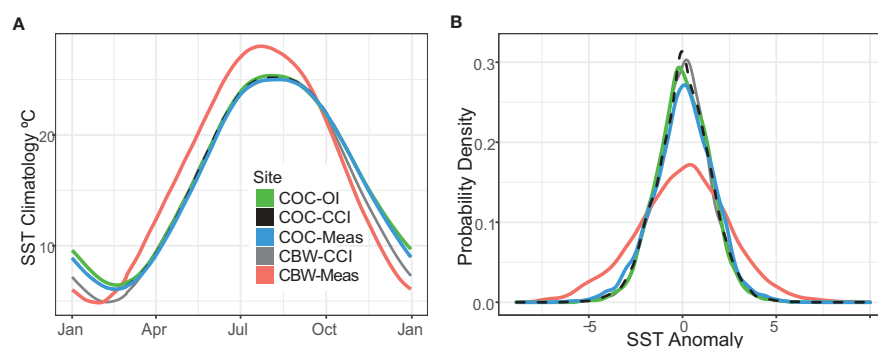
FIGURE 2 Statistics of SST time series at the bay and coastal ocean sites. (A) 30-year seasonal climatology for gridded (OI, CCI) and measured (Meas) time series at the coastal ocean (COC) and coastal bay (CBW) sites. (B) Probability distribution of SST anomaly for each site; colors as in (A).
