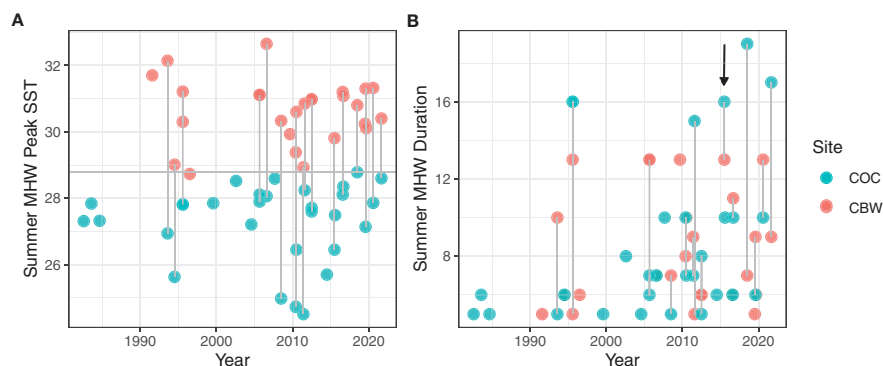
FIGURE 4 Summer MHW peak SST and duration. (A) Peak MHW SST during summer (June, July, August) and (B) MHW duration for the coastal ocean (COC, blue) and bay (CBW, red) sites. Each pair of points connected by a vertical line represents a MHW that occurred simultaneously at both sites. The horizontal line in (A) at SST=28.8°C separates peak ocean and bay peak MHW temperatures in summer. The black arrow in (B) points to the June 2015 MHW.
