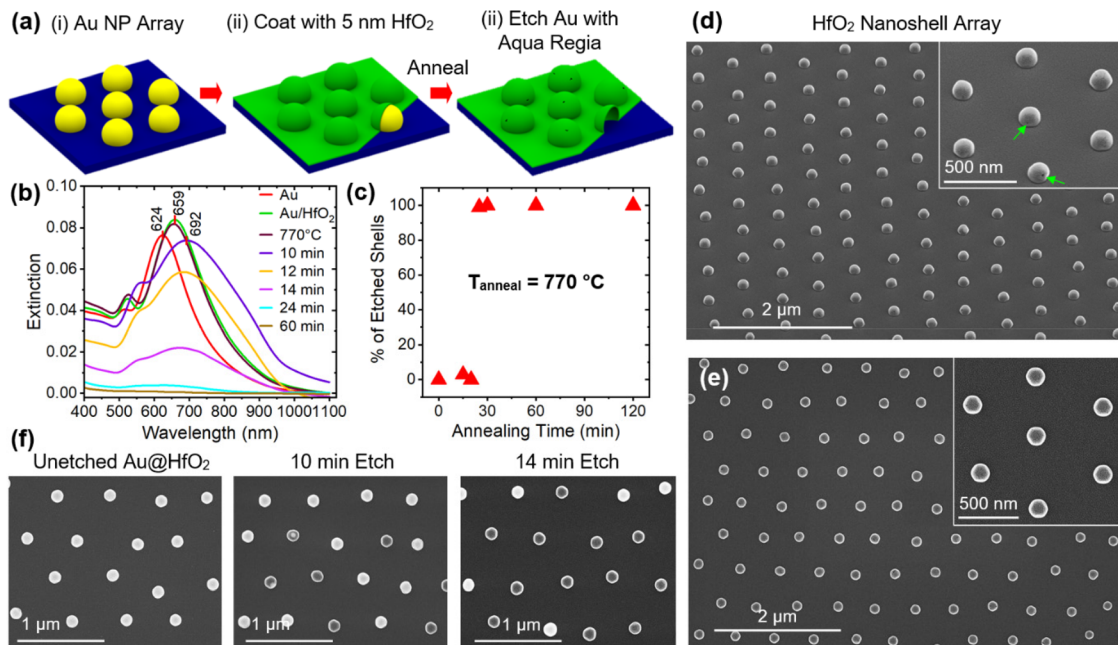
Fig. 1 (a) Schematic depicting the three-stage procedure for forming periodic arrays of air-filled HfO 2 nanoshells. Note that the bottom right corner of the second- and third-stage schematics show HfO 2 cutaways revealing the internal structure of the nanoshells. (b) Extinction spectra obtained as the Au NP array is coated with HfO 2 , annealed at 770 °C for 30 min, and then exposed to an aqua regia etch for various time intervals. (c) Plot showing the percentage of successfully etched nanoshells as a function of anneal time. (d) Tilted- and (e) top-view SEM images of a HfO 2 nanoshell array formed under optimum conditions. (f) Top-view SEM images showing the Au etching process at various stages where bright and dark NPs correspond to unetched and fully etched nanoshells, respectively. Note that the array shown in (e) provides an image of the fully etched structures.
