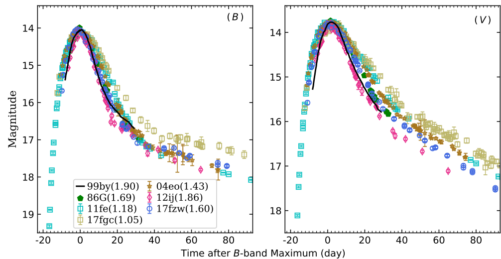
Figure 4. BV -band light curves of SN 2017fzw from LCO, compared with SNe 1999by (91bg-like subgroup), 2011fe, 2017fgc (normal subgroup), 2004eo, 1986G, and 2012ij (transitional subgroup). The values in brackets represent the light curve shape parameter ( \Delta m_{15}(B) ) [27,28]. All light curves of comparison SNe Ia have been shifted to match SN 2017fzw in magnitudes of the maximum.
