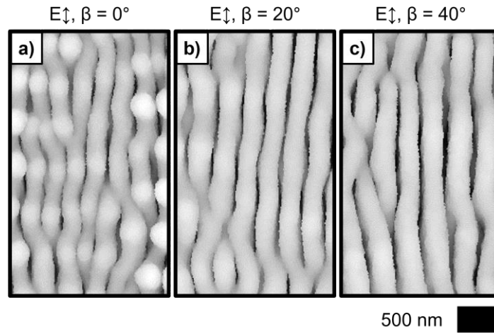
Figure 3. Simulated deposit morphologies generated via growth modeling with vertically polarized ( E \uparrow ) \lambda_{\text{avg}} = 626 nm illumination with the indicated inclination ( \beta ) from the substrate normal in the plane of the polarization.
