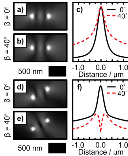
Figure 4. (a) Simulation of the normalized time-average electric field magnitude from two coherent dipole sources emitting radiation with a free space wavelength of \lambda = 626 nm in a medium of refractive index n = 1.33 . The dipole oscillation axis was along the vertical and the dipoles were separated by one wavelength along the horizontal. (b) Same as (a) but with the dipole oscillation axis inclined 40^\circ into the simulation plane. (c) Line profiles of the field magnitude from the simulations in (a) and (b) along the axis along perpendicular to the separation axis and through the separation midpoint. (d) and (e) Same as (a) and (b), respectively, but with the dipole sources separated along a diagonal axis. (f) Similar line profiles as in (c) but corresponding to the simulations in (d) and (e).
