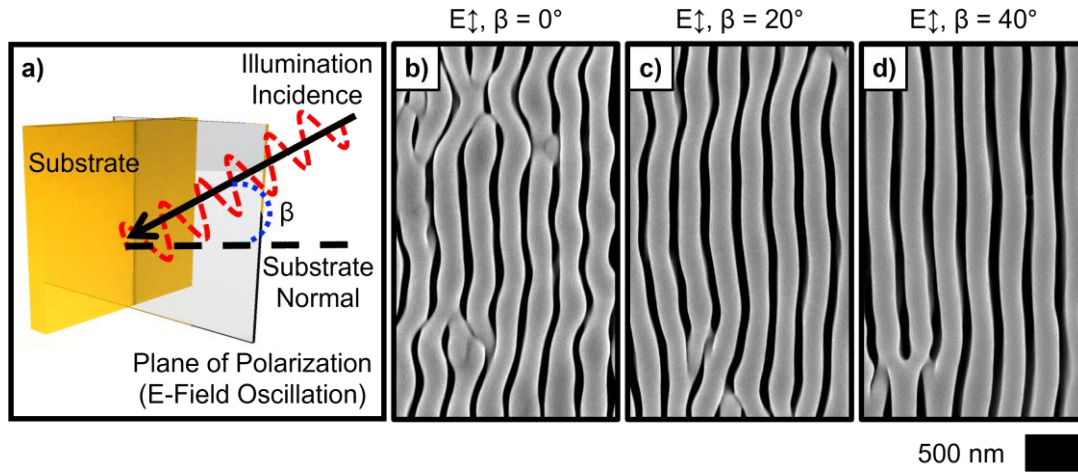
Figure 1. (a) Schematic illustration of electrode substrate illumination with linearly polarized light inclined in the plane of the polarization. (b)–(d) Representative SEMs of deposits generated with vertically polarized ( E \uparrow ) \lambda_{\text{avg}} = 626 nm illumination with the indicated inclination ( \beta ) from the substrate normal in the plane of the polarization.
