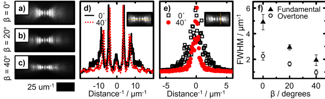
Figure 2. (a)-(c) 2D FTs generated from SEM data of the deposits depicted in Figure 1(b)-(d) respectively. (d) Fourier spectra representing the intensity along the horizontal centerlines of the 2D FTs depicted in (a) and (c). (e) Fourier spectra representing the intensity along the vertical centerlines of the positive fundamental modes in the 2D FTs in (a) and (c). (f) FWHM of fit curves of spectral profiles similar to those in (e) for the positive fundamental and first overtone modes in the 2D FTs in (a)-(c) as a function of \beta .
