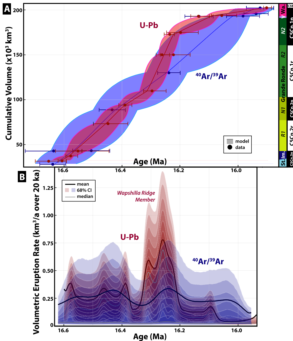
Fig. 3. CRBG U-Pb and ^{40}\text{Ar}/^{39}\text{Ar} age models. A) U-Pb (red) and ^{40}\text{Ar}/^{39}\text{Ar} (blue) age models for cumulative volume erupted through the CRBG. Input data for the models are U-Pb eruptive ages after Keller et al. (2018) and ^{40}\text{Ar}/^{39}\text{Ar} dates with 2\sigma analytical uncertainty. Shading indicates 95% credible interval of the models, with internal uncertainties only. The position of the Vantage sedimentary interbed is labeled with “V”. B) Results from (A) were used in further MCMC simulation to calculate average long-term emplacement rates through the eruptive history of the CRBG, averaged over 20 kyr windows, shown with contours up to the 68% credible interval (CI).
