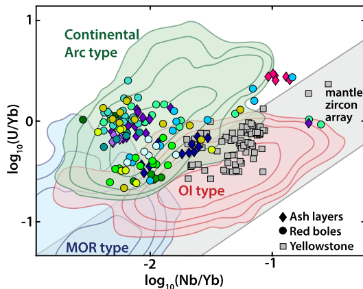
Fig. 7. CRBG zircon provenance. Tectono-magmatic zircon provenance diagram after Grimes et al. (2015), outlining fields for mid-ocean ridge (MOR type), ocean island and other plume-influenced (OI type), and continental arc type zircons. CRBG zircons analyzed are color-coded by sample, with lithology identified by shape, and are compared to \sim 100 ka zircons analyzed from Yellowstone volcanics by Stelten et al. (2013).
