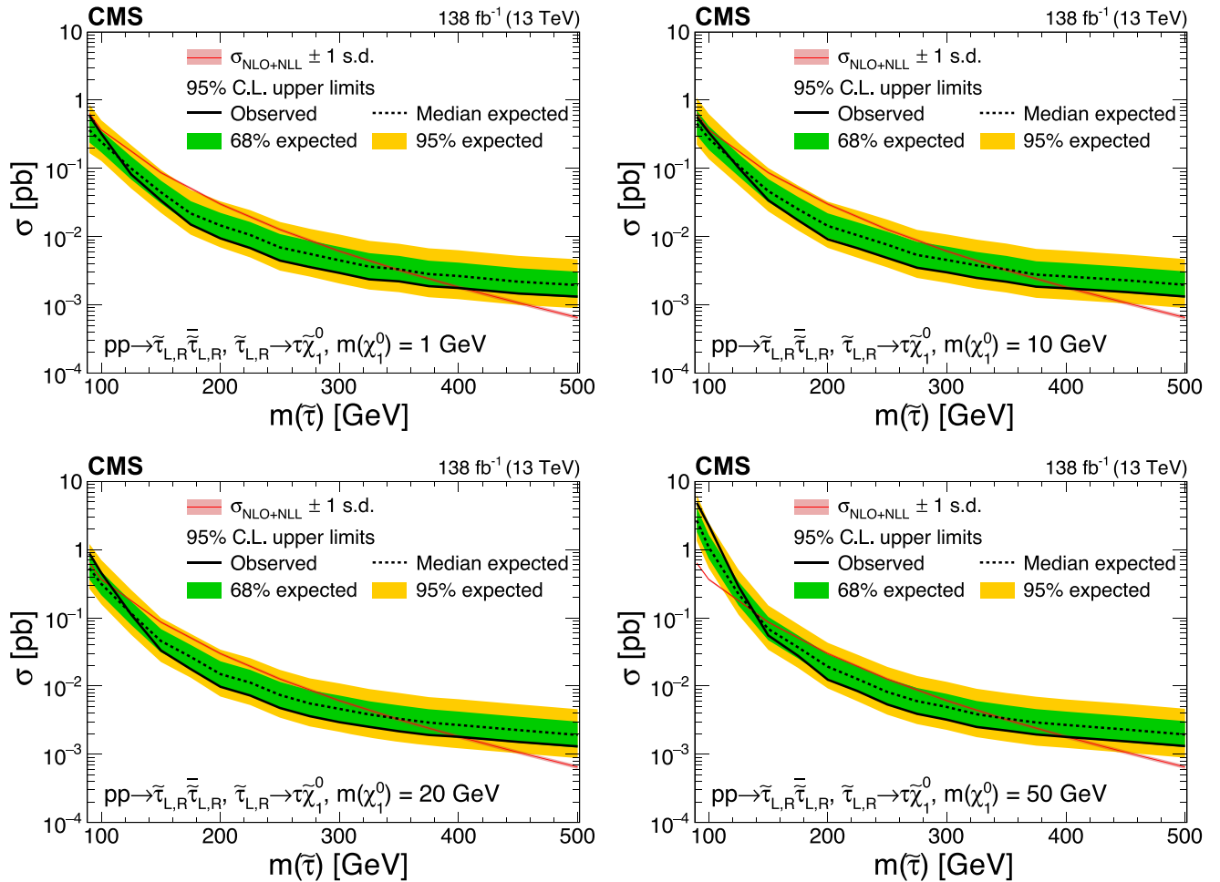
FIG. 4. Expected and observed 95% CL cross section upper limits as functions of the \tilde{\tau} mass in the degenerate \tilde{\tau} scenario for \tilde{\chi}_1^0 masses of 1, 10, 20, and 50 GeV (upper left to lower right). The inner (green) band and the outer (yellow) band indicate the regions containing 68% and 95%, respectively, of the distribution of limits expected under the background-only hypothesis. The red line and thin shaded band indicate the NLO + NLL prediction for the signal production cross section calculated with RESUMMINO [30,62], and its uncertainty.
