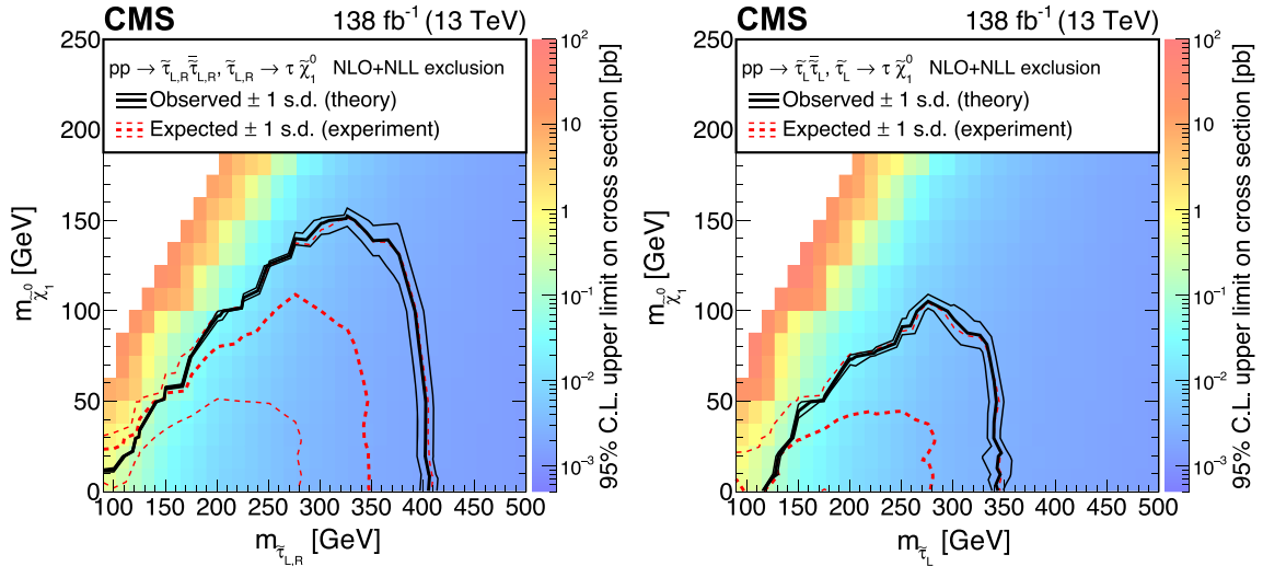
FIG. 7. Upper limits at 95% CL on the cross section for degenerate (left) and purely left-handed (right) \tau pair production in the m(\tau) - m(\tilde{\chi}_1^0) plane. The thick black (red) curves show the observed (expected) exclusion limits assuming NLO + NLL predictions for the signal cross sections. The thin black curves represent the variations in the observed limits obtained when these cross sections are varied by their \pm 1 standard deviation uncertainties. The thin dashed red curves indicate the region containing 68% of the distribution of limits expected under the background-only hypothesis.
