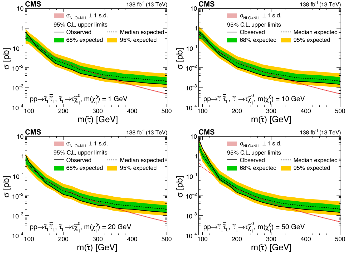
FIG. 5. Expected and observed 95% CL cross section upper limits as functions of the \tau mass in the purely left-handed \tau scenario for \chi_1^0 masses of 1, 10, 20, and 50 GeV (upper left to lower right). The inner (green) band and the outer (yellow) band indicate the regions containing 68% and 95%, respectively, of the distribution of limits expected under the background-only hypothesis. The red line and thin shaded band indicate the NLO + NLL prediction for the signal production cross section calculated with RESUMMINO [30], and its uncertainty.
