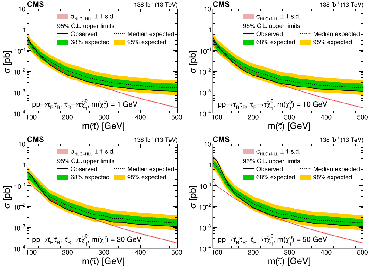
FIG. 6. Expected and observed 95% CL cross section upper limits as functions of the \tau mass in the purely right-handed \tau scenario for \tilde{\chi}_1^0 masses of 1, 10, 20, and 50 GeV (upper left to lower right). The inner (green) band and the outer (yellow) band indicate the regions containing 68% and 95%, respectively, of the distribution of limits expected under the background-only hypothesis. The red line and thin shaded band indicate the NLO + NLL prediction for the signal production cross section calculated with RESUMMINO [30], and its uncertainty.
