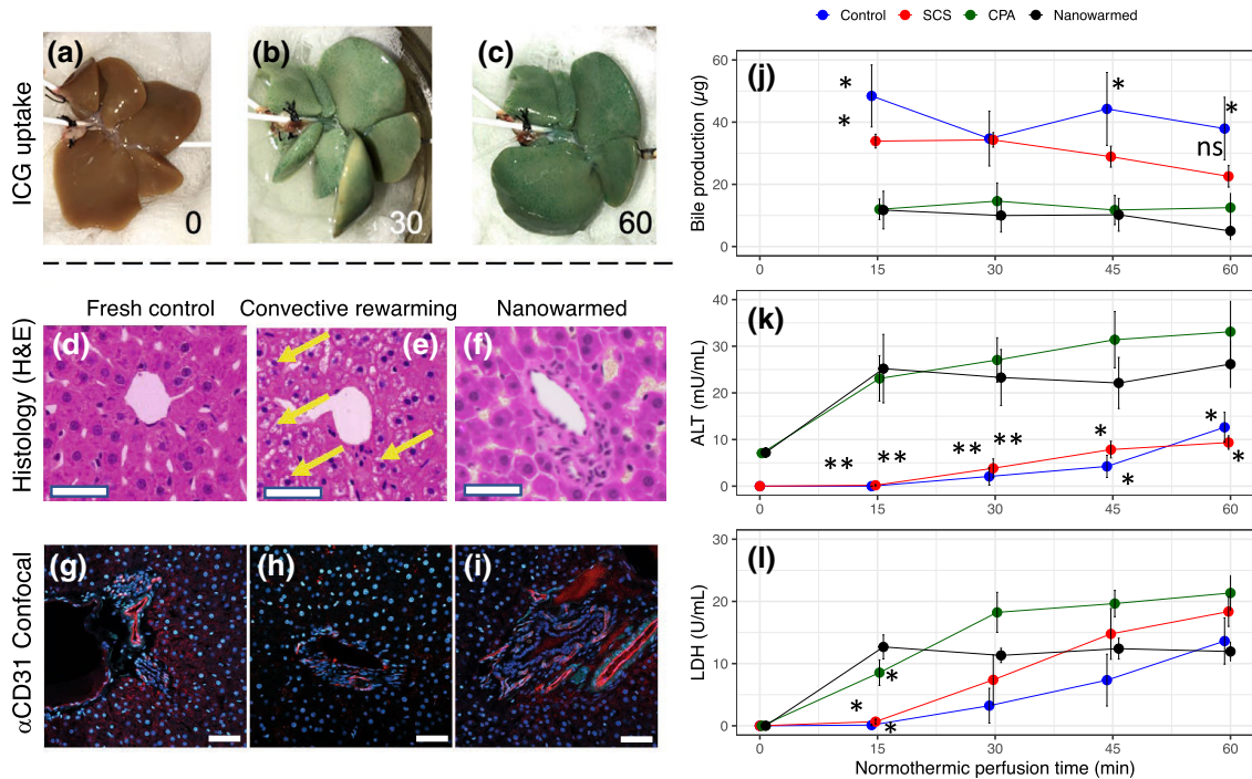
FIGURE 5. Organ-level function in vitrified and nanowarmed livers. Vitrified and nanowarmed livers were tested for function and injury as compared to static cold storage (SCS, 18–20 h in UW solution at 4 °C), CPA loaded and unloaded but not vitrified and untreated (flushed with UW and used within 30 min) controls. (a–c) Following washout of CPA + sIONP, the organs were assessed by normothermic machine perfusion with indocyanine green (ICG) in the perfusate and imaged at 0, 30, and 60 min. The nanowarmed livers demonstrated organ-level function with homogenous ICG uptake. (d–f) Histologic examination (hematoxylin and eosin) of control (left), vitrified and convectively rewarmed (middle), and vitrified and nanowarmed (right) livers show preserved tissue architecture in nanowarmed livers. Convectively rewarmed livers had diffuse areas of extra- and intracellular white space (yellow arrows) suggestive of ice crystallization during rewarming or cytoplasmic vacuolization. Nanowarmed livers have a normal portal and sinusoidal architecture. Bar = 100 \mu m. (g–i) Confocal imaging with anti-CD31 immunofluorescence shows that control and nanowarmed livers have preserved vascular architecture (red staining), whereas convectively rewarmed livers have reduced staining intensity, indicating endothelial injury. (j) Bile production assessed during 60 min of normothermic perfusion after nanowarming was not different than CPA-loaded and unloaded livers. Hepatocyte injury was assessed by measuring ALT (k) and LDH (l) in the SHVC venous effluent during perfusion. ALT levels for nanowarmed livers were slightly higher than for control organs throughout the normothermic perfusion, whereas LDH levels were not different between nanowarmed livers and other groups after 15 min. For all groups, n = 3 –5. p values show comparison to nanowarming only with * p < 0.05 and ** p < 0.01 . All significant differences are shown. Full pairwise comparison statistics are in Supplementary Materials.
