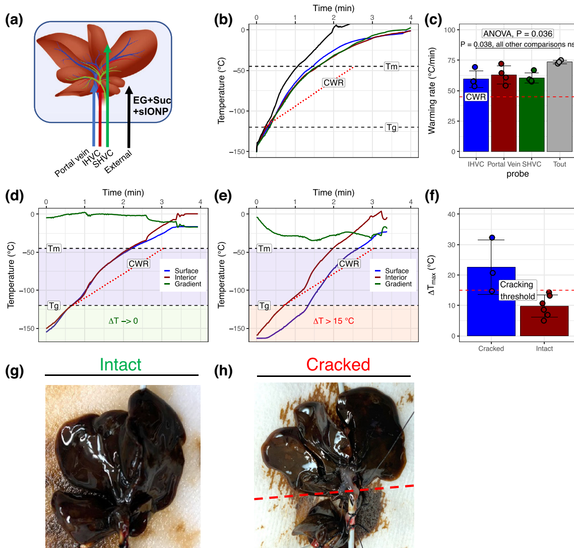
FIGURE 4. Rewarming of CPA and sIONP-loaded vitrified livers. (a) Positioning of fluoro-optic temperature probes within and around the liver. (b) Temperature vs. time recordings during nanowarming of vitrified rat livers show rewarming at rates exceeding the CWR of CPA (EG + suc) in all liver regions (c). (e) During initial testing, rewarming was initiated from -150^\circ\text{C} at high power (63 kA/m, 185 kHz, right panel). A significant temperature difference (gradient) between the IHVC and the solution around the liver developed rapidly. This difference persisted through the glassy temperature zone (i.e., < T_g , red box), where the system is subject to thermal stress-induced cracking. Under these conditions, visible and audible cracking occurred in the livers (h). (d) When the RF coil energy was initiated at low power between -150^\circ\text{C} and -115^\circ\text{C} (above T_g , green box), temperature differences were much lower and cracking did not occur (g). (f) The measured temperature differences from several experiments were compiled and correlated with the presence or absence of liver cracking. A cutoff of 15^\circ\text{C} was defined as the threshold for cracking. Data are mean \pm SD ( n = 3\text{--}6 per group).
