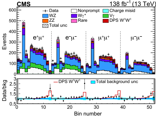
FIG. 2. Postfit distribution of the final BDT discriminant output for the four lepton flavor and sign categories. The SPS W^\pm W^\pm , t\bar{t}V , and VVV contributions are grouped as the “rare” background. The total postfit uncertainty in the signal and background predictions is shown as the hatched band. The bottom panels show the ratio of data to the sum of all background contributions as the black data points along with the extracted signal shown by the red line. The vertical error bars on the data points represent the statistical uncertainty of the data.
