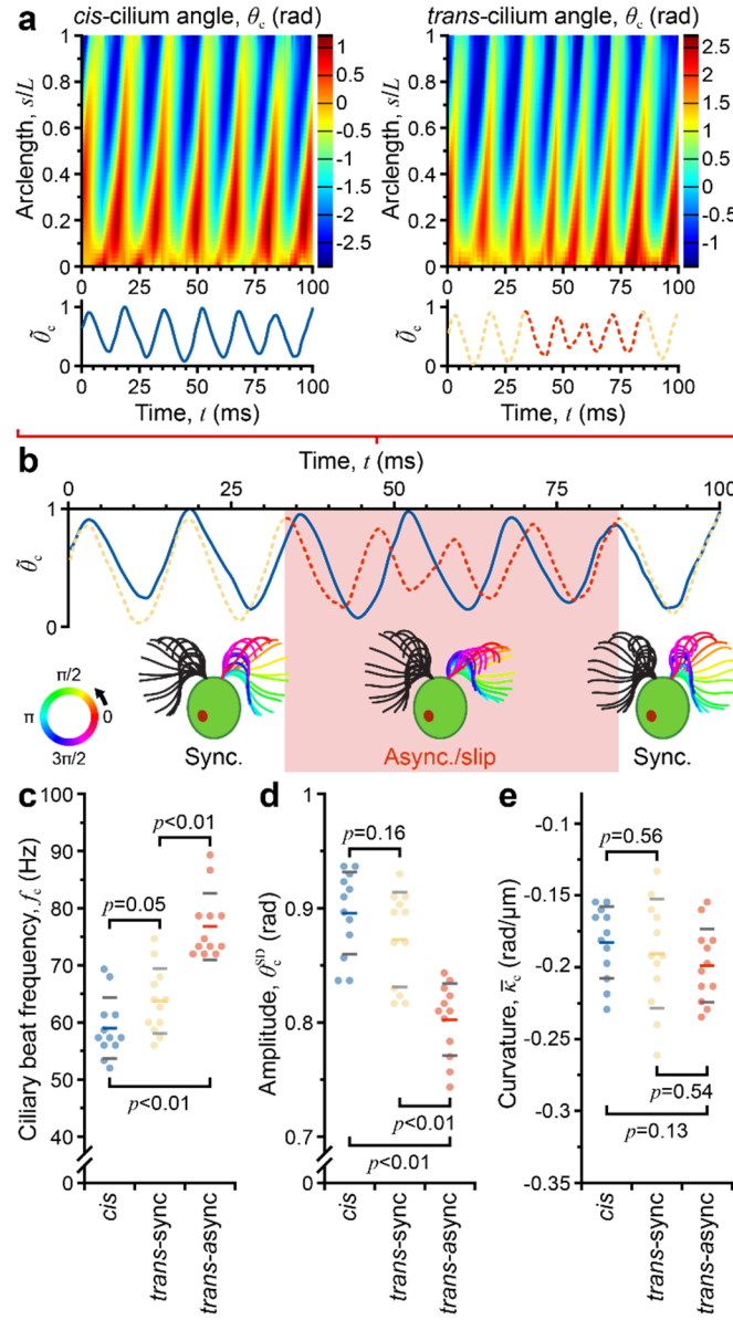
Figure 3. Characterization of ciliary beat asynchrony during long-term acoustic trapping. (a) Beat periodicity using normalized average cilium angle \bar{\theta}_c vs time [average determined from map of \theta_c vs. nondimensional space (arclength s/L ; y -axis) and time ( x -axis)]. (b) Identification of cis-trans beat asynchrony. (c)-(e) Comparison of ciliary waveform parameters beat frequency f_c , amplitude \theta_c^{SD} , and mean curvature \bar{\kappa}_c for synchronous and asynchronous beating.
