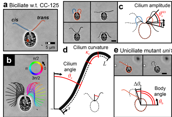
Figure 2. Schematics of biciliate wild-type (strain CC-125) and uniciliate mutant (strain uni1 ) Chlamydomonas reinhardtii cells held in the acoustic tweezers. (a) Identification of cis and trans cilia for biciliate cells. (b) Ciliary shapes at equidistant times representing a complete beat cycle ( t \approx 17 ms). (c) and (d) Definitions of cilium amplitude, angle, and curvature. (e) Definition of body angle for uni1 cells.
