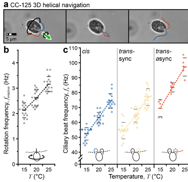
Figure 4. Measurement of 3D body rotation. (a) Sequence of images following one body inversion (half of a complete rotation). (b) and (c) Comparison of C. reinhardtii body rotation rate f_{\text{rotation}} and ciliary beat frequency f_c with increasing temperature T .
