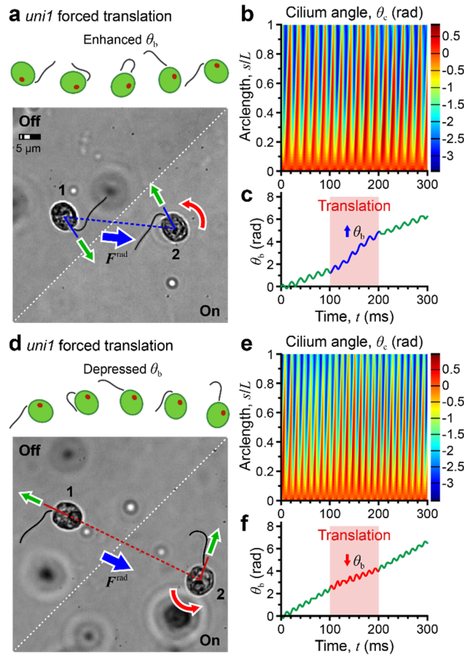
Figure 6. Acoustic perturbation for rapid translation of the cell body. (a)-(c) Cell axis aligned with the acoustic radiation force, enhancing the rotation rate of the cell body. (d)-(f) Cell axis oriented opposite the acoustic radiation force, depressing the rotation rate.
