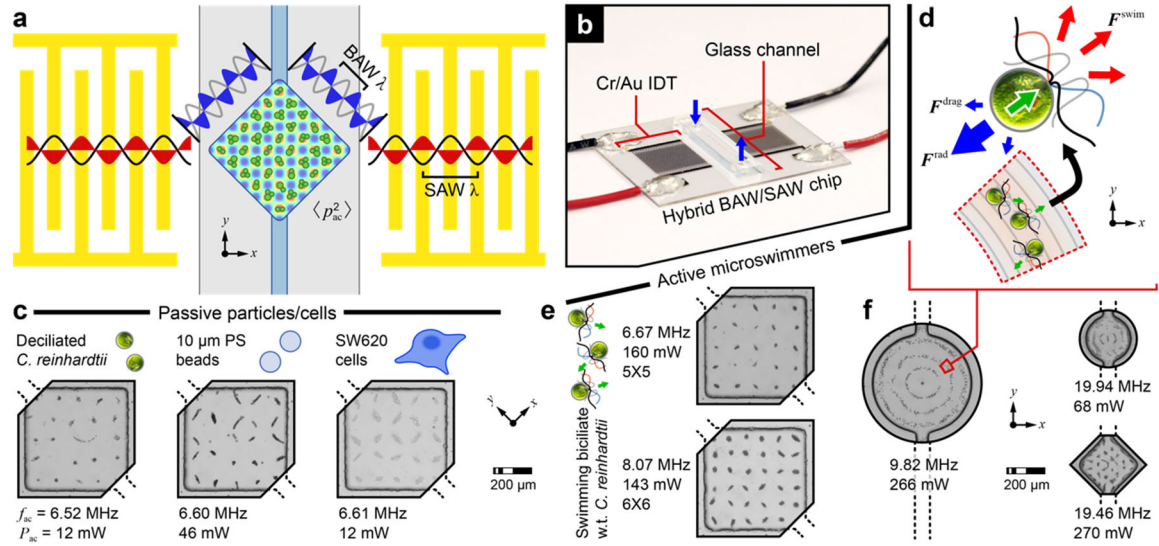
Figure 1. Acoustic tweezers incorporating two-dimensional (2D) bulk acoustic waves (BAW) driven by one-dimensional (1D) surface acoustic wave (SAW) actuation. (a) Illustration of hybrid BAW/SAW device for patterning cell populations and trapping single-cell microswimmers, and (b) assembled device. (c) Patterning of various passive particles/cells. (d)-(f) Microswimmer confinement to acoustic potential minima of BAW fields driven by SAW actuators. Note that the internodal spacing of the 2D patterns reflects the wavelength of BAW at the reported actuation frequencies.
