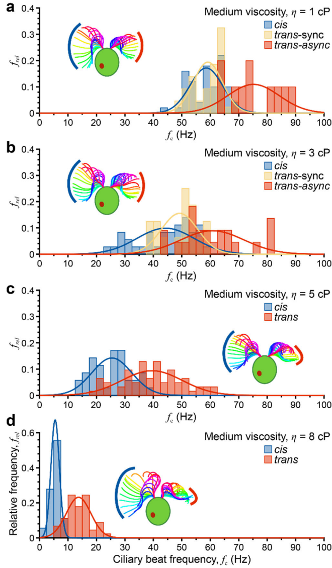
Figure 5. Effect of viscosity on ciliary beat synchrony. (a)-(d) As medium viscosity is increased from \eta = 1 cP to \eta = 8 cP, synchronization decreases until only asynchronous beating is observed for \eta \geq 5 cP. Note f_{rel} is the relative frequency of occurrence of cells with a particular beat frequency.
