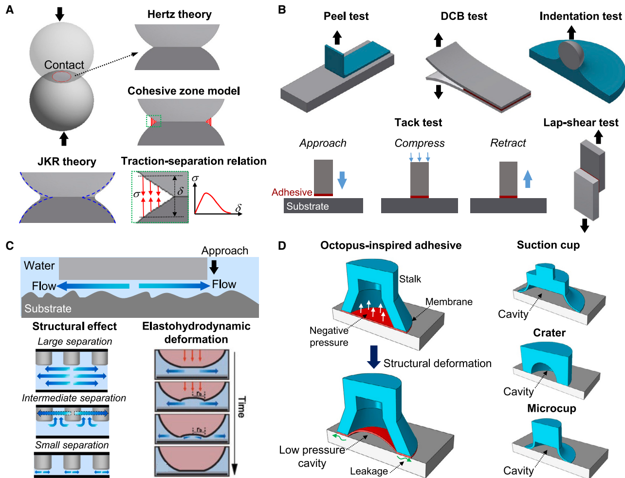
Figure 4. Modeling and testing underwater adhesion
