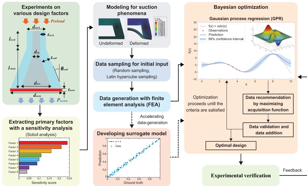
Figure 5. Workflow chart for data-driven adhesive design
