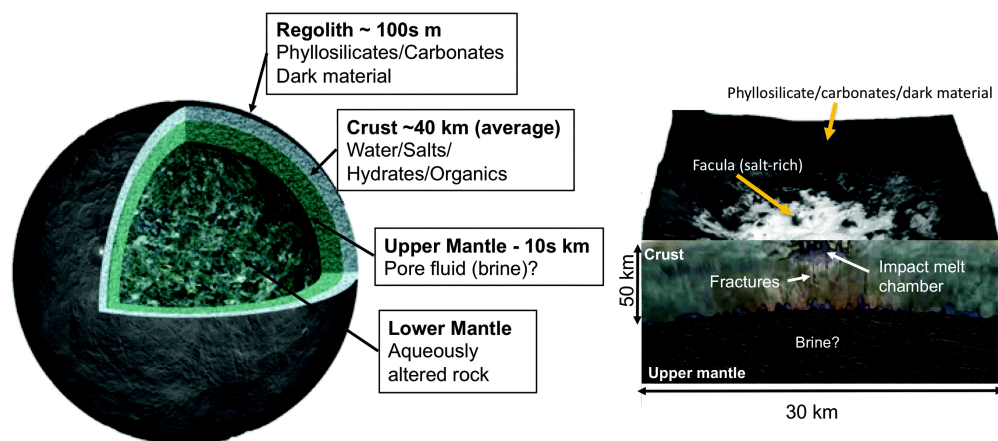
FIG. 2. Left: Global interior structure for Ceres: a ~40-km thick (average) strong crust is composed of rock+ice+salts+clathrates with no more than ~40% ice (Bland et al. , 2016; Ermakov et al. , 2017a; Fu et al. , 2017). It overlays a rocky mantle with a weak upper layer with brine-filled pore space that controls the global shape (Fu et al. , 2017). Right: Possible structure of the crust inferred below Occator Crater's faculae, in a region where the crust is ~50 km thick (Ermakov et al. , 2017a). Impact craters could create transient melt chambers. Large impacts could also introduce or re-enact fractures allowing for the upwelling of deep brines. This rendition assumes that the impact melt reservoir was originally larger in extent but is mostly frozen at present, except for brines supplied from the deeper reservoir (Hesse and Castillo-Rogez, 2019). (Credit: NASA/JPL-Caltech/UCLA/MPS/DLR/IDA for the Occator image; crust rendition modified from Britney Schmidt/Dead Pixel FX/Univ. of Texas at Austin.).
