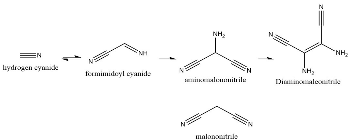
Figure 1. Self-polymerization of hydrogen cyanide (HCN). Under hydrothermal conditions and high concentrations, HCN polymerization of the monomer into the dimer (iminoacetoneitrile) is spontaneous and reversible. Polymerization to the trimer (aminomalononitrile) and further into the tetramer (DAMN) is also spontaneous but is not a reversible reaction. Note the comparison of aminomalononitrile ( above ) to malononitrile ( below ) and the lack of an amine group on the second carbon of malononitrile.
