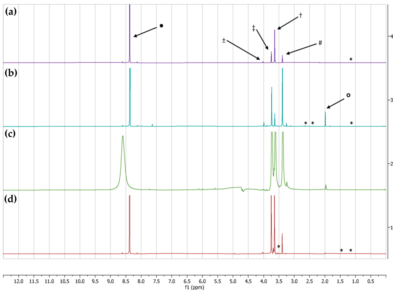
Figure 9. Selected ^1\text{H} -NMR spectra of malononitrile after 48 h at 90 °C: (a) malononitrile and sodium formate; (b) malononitrile, sodium formate, and rhodium; (c) malononitrile, sodium formate, and FeS; (d) malononitrile, sodium formate, and \text{Al}_2\text{O}_3 . Major suspected hydrolysis product peaks are: \pm = malononitrile, \dagger = malonamide, \# = malonate (malonic acid), \ddagger = malonic acid monoamide, and \circ = amide functional group. \bullet = sodium formate. * = multiplet locations. Expanded spectra with detailed chemical shifts and multiplet locations can be found in Figures S2–S5.
