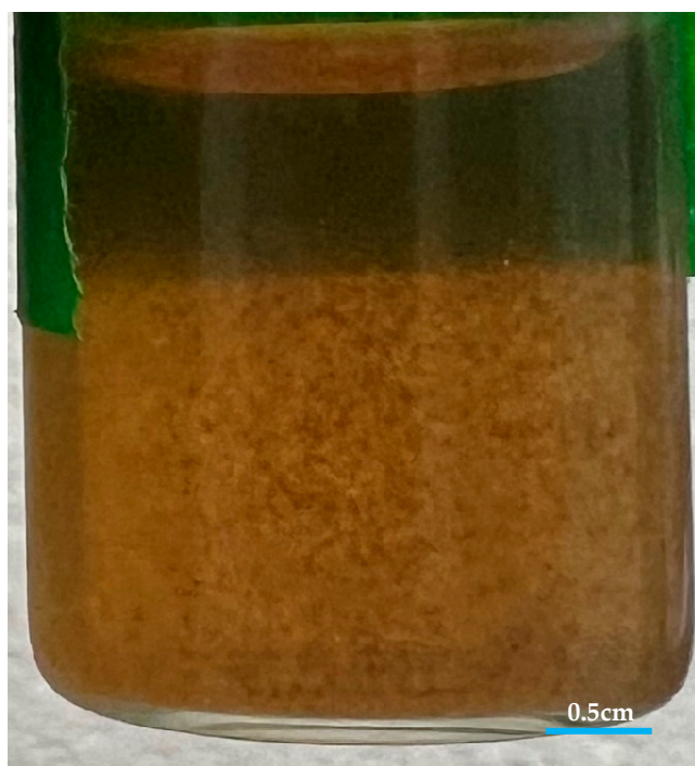
Figure 2. Malononitrile incubated for 48 h at 90 °C with sodium formate. The uneven coloring is suspended insoluble polymer. A 0.5 cm scale bar is included for reference.
