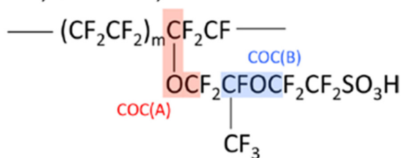
Fig. 7 Molecular structure of perfluorosulfonated ionomer (Nafion). Reproduced from ref. 95 with permission from [American Chemical Society], copyright [2014].
