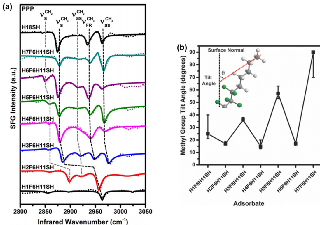
Fig. 14 Data obtained from H n F6H11SH fluorinated SAMs series. (a) Normalized SFG spectra for the C–H stretching region. The solid lines denote the fits to the spectra according to eqn (1). PPP denotes the polarization direction of the SFG, visible, and IR beams in that order with respect to the surface normal. The symmetric ν s CH 3 , and antisymmetric ν as CH 3 methyl C–H stretching peak positions are marked with black dotted lines. (b) Average methyl group tilt angle of the H n F6H11SH fluorinated SAMs, derived from the SFG spectra. Reproduced from ref. 4 with permission from [American Chemical Society], copyright [2020].
