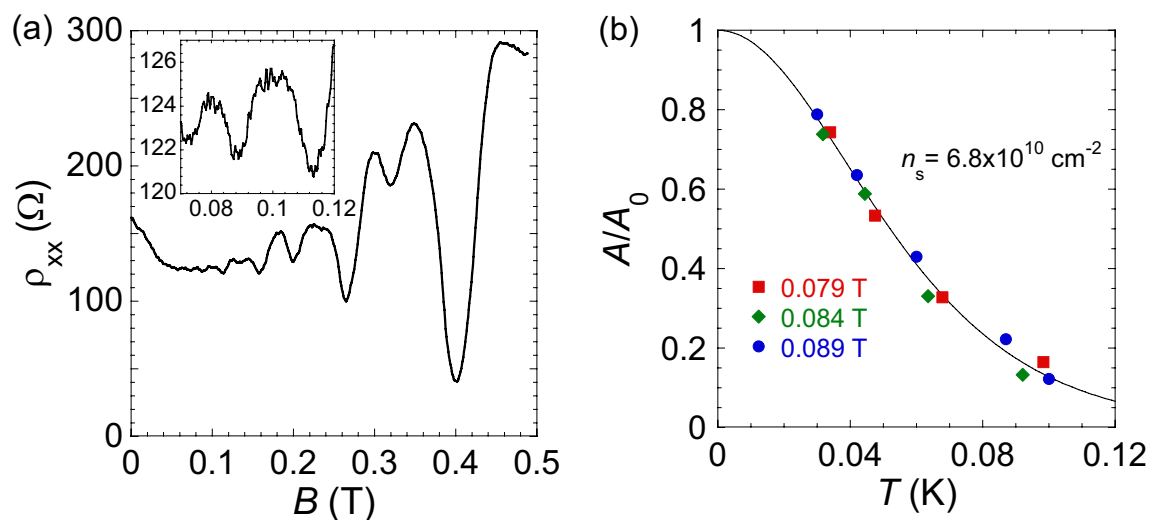
Figure 1. (a) Shubnikov-de Haas oscillations in perpendicular magnetic fields at T = 30 mK and n_s = 3.97 \times 10^{10} cm -2 . A fragment of the weak-field SdH oscillations averaged over 32 traces is shown in the inset. (b) Change of the amplitude of the weak-field SdH oscillations in perpendicular magnetic fields with the temperature at n_s = 6.8 \times 10^{10} cm -2 and B_1 = 0.079 T (squares), B_2 = 0.084 T (diamonds) and B_3 = 0.089 T (circles). The values of T for the data obtained in B_1 and B_2 are multiplied by B_3/B_1 and B_3/B_2 , correspondingly. The solid line is a fit using Eq. (1).
