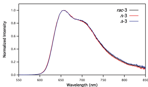
Fig. 5 Normalized emission spectra of the rac - 3 and the \Lambda - 3 , \Delta - 3 enantiomers as powder at room temperature.
