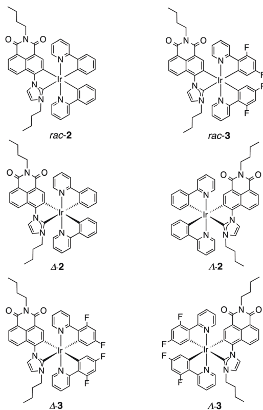
Fig. 1 Complexes described in this work.
