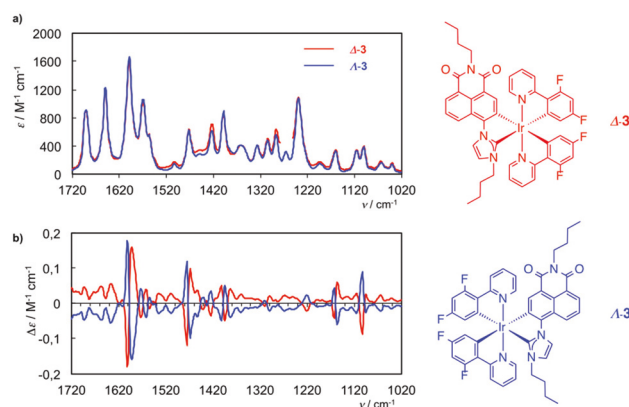
Fig. 6 Experimental IR (a) and (b) VCD spectra of complex \Delta - 3 (red) and \Lambda - 3 (blue) in \text{CD}_2\text{Cl}_2 . The half-sum has been used as the baseline.
