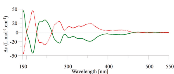
Fig. 2 CD spectra of \Delta -2 (green) and \Lambda -2 (red) recorded in \text{CH}_3\text{CN} at 0.19 mM.
