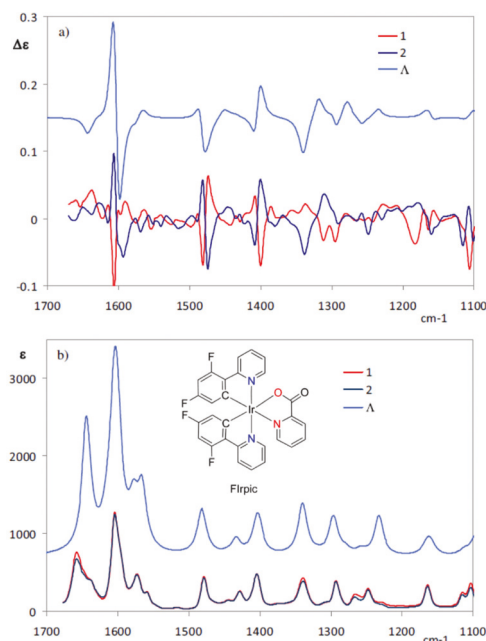
Fig. 7 Comparison of experimental VCD (a) and experimental IR (b) spectra enantiomers 1 and 2 of Flrpic with the corresponding calculated spectra of the \Delta enantiomer. Adapted from reference. 30
