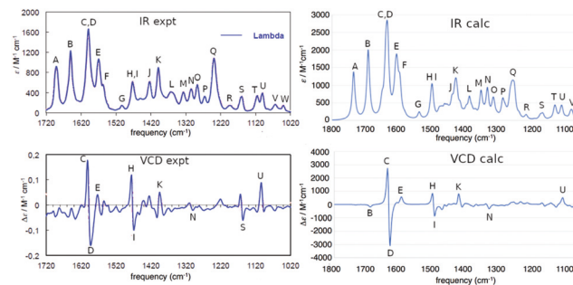
Fig. 8 Experimental (left) and Calculated (right) Harmonic IR and VCD Spectra for \Delta - 3 between roughly 1000 \text{cm}^{-1} and 1800 \text{cm}^{-1} .
