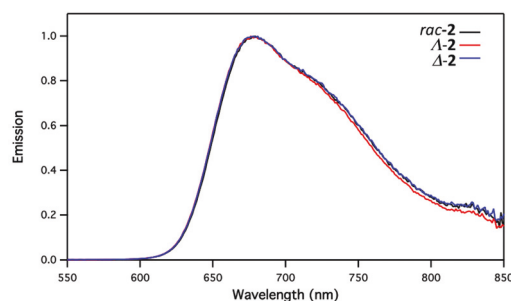
Fig. 4 Normalized emission spectra of the rac - 2 and the \Lambda - 2 , \Delta - 2 enantiomers as powder at room temperature.
