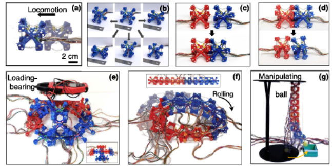
Fig. 1. Starbots: (a) Locomotion of a single module; (b) Five deformation primitives of a single module; (c) Attachment of a pair of modules; (d) Detachment of a pair of modules; (e) Formation and weight-carrying of a 3D dome-shaped tent; (f) Locomotion of a modular rolling robot; (g) Object manipulation of a module-based robotic arm and gripper.
