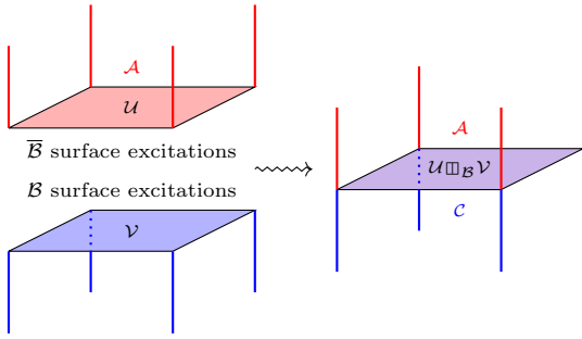
FIG. 6. Taking K_B -modules in \mathcal{U} \boxtimes \mathcal{V} glues the Witt-equivalences {}_{\mathcal{A}}\mathcal{U}_B and {}_B\mathcal{V}_C to obtain the Witt-equivalence {}_{\mathcal{A}}(\mathcal{U} \boxtimes_{\mathcal{B}} \mathcal{V})_C .
