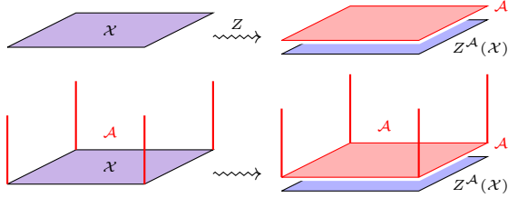
FIG. 5. Since Z(\mathcal{X}) \cong Z^{\mathcal{A}}(\mathcal{X}) \boxtimes \mathcal{A} , attaching an \mathcal{A} -Walker-Wang bulk to \mathcal{X} trivializes the \mathcal{A} -layer of topological order, leaving only Z^{\mathcal{A}}(\mathcal{X}) .
