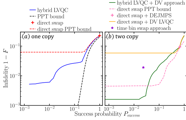
Figure 3. Infidelity of transmon qubits versus success probability on (a) one-copy and (b) two-copy entangling microwave modes with C = 0.1, n_{\text{in}} = 0.2, \zeta_{\text{m}} = 0.992, \zeta_{\text{o}} = 0.99 . The PPT bound (black) in (a) goes below 10^{-4} and saturates; red and pink dashed curves in (a)(b) correspond to PPT bound of one-copy and two-copy two-qubit state by direct swap. There are D = 10 ECD blocks in hybrid LVQCs and L = 6 layers in DV LVQCs.
