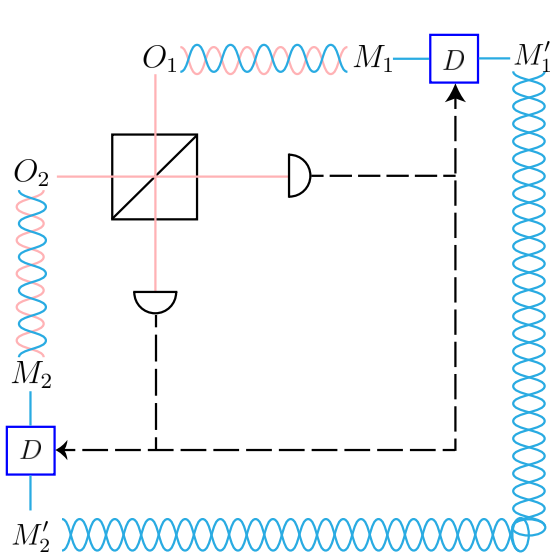
Figure 5. Continuous-variable entanglement swap scheme. The cavities generate two entangled mode pairs O_1M_1 and O_2M_2 . Then two optical modes O_1 and O_2 are mixed by a balanced beam splitter. We perform homodyne measurements at the output of beam splitter and then displace the microwave modes M_1 and M_2 , producing two entangled microwave modes M_1' and M_2' .
