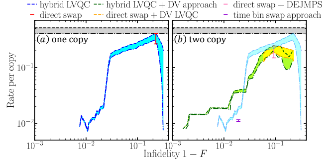
Figure 4. Entanglement distillation rate per copy on (a) one-copy and (b) two-copy noisy entangled microwave modes versus infidelity 1-F , at identical parameters to Fig. 3. Dot-dashed and dashed curves correspondingly represent RCI lower bounds and EoF upper bounds. Shaded areas and line segments show the range of rate. The shallow blue curves and areas in (b) are same as (a) for comparison.
