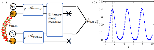
Figure 10. (a) Schematic of the direct swap approach. (b) Entanglement of formation E_f between qubits versus evolution time t . Vertical dashed line indicates the time with maximum entanglement at t = \pi/2 .
