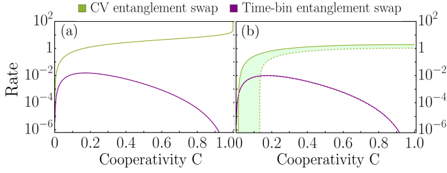
Figure 2. Rate (in ebit per round) comparison (a) \zeta_m = \zeta_o = 1 . (b) \zeta_m = 0.95 , \zeta_o = 0.9 and n_{in} = 0.2 . The rate of CV entanglement swap is within green shaded and the rate of time-bin entanglement swap is within purple region.
