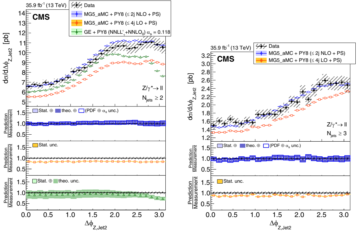
FIG. 19. The measured differential cross section as a function of the Z boson and subleading jet azimuthal difference for events with at least two (left) and three (right) jets. The measurement statistical (resp. systematic) uncertainties are represented with vertical error bars (resp. hashed areas). The measurement is compared to the NLO MG5_aMC, LO MG5_aMC, and GENEVA (for N_{jets} \geq 2 ) predictions described in Sec. VI. The predictions uncertainties, estimated as explained in this section, are represented by colored areas in the ratio plots (light color for the statistical part and darker color for the total). Only the statistical uncertainty is displayed for the LO prediction.
