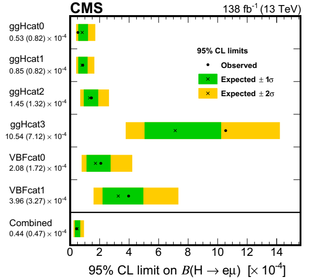
FIG. 5. Observed (expected) 95% CL upper limits on \mathcal{B}(H \rightarrow e\mu) for each individual analysis category (as shown in the left axis label) and for the combination of all analysis categories.
