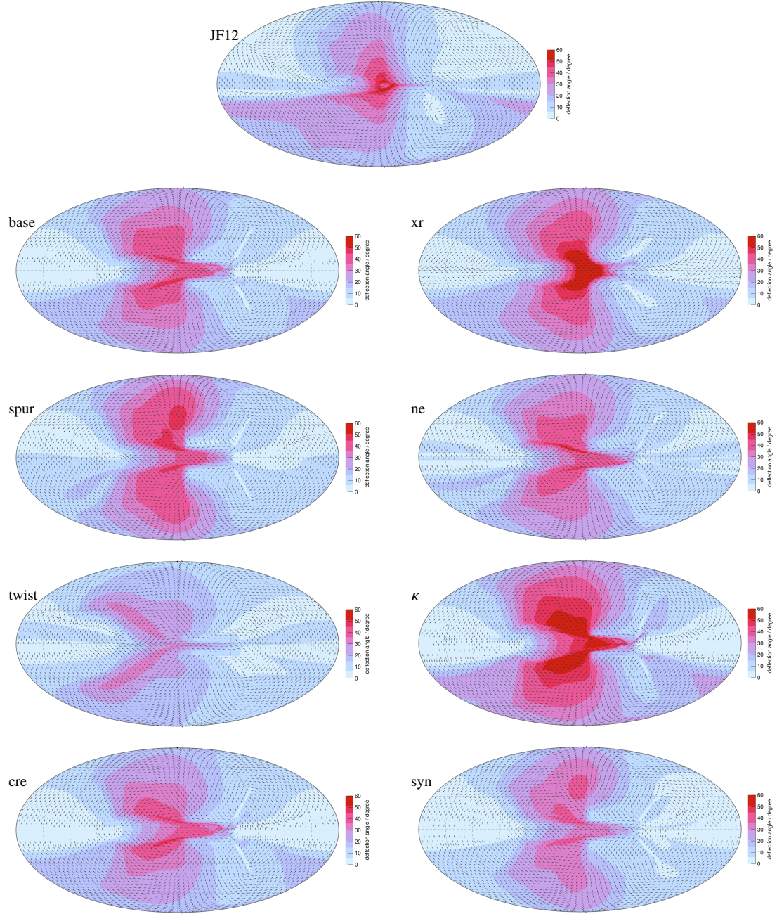
Figure 1: Angular deflections of ultrahigh-energy cosmic rays in JF12 model (top) and the eight model variations derived in this paper. Arrows and colors illustrate the size and direction of the deflection in the GMF following the particles from Earth to the edge of the Galaxy. Positions denote on the sky map arrival directions at Earth. The rigidity is 20 EV.
