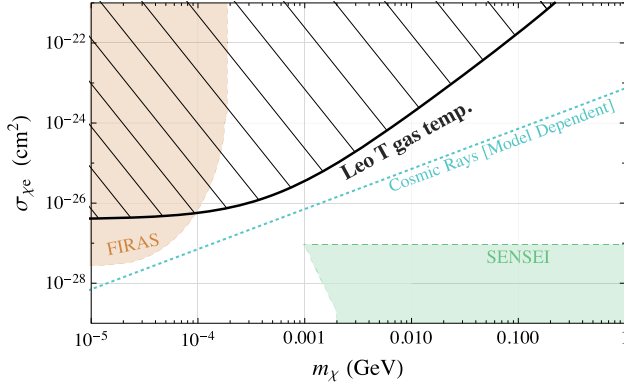
FIG. 9. Upper bounds on velocity-independent DM-free electron scattering from Leo T (black), FIRAS (brown) [161], and indirect, model-dependent bounds from cosmic rays [162] (cyan). The exclusion region from SENSEI [117] is also shown.
