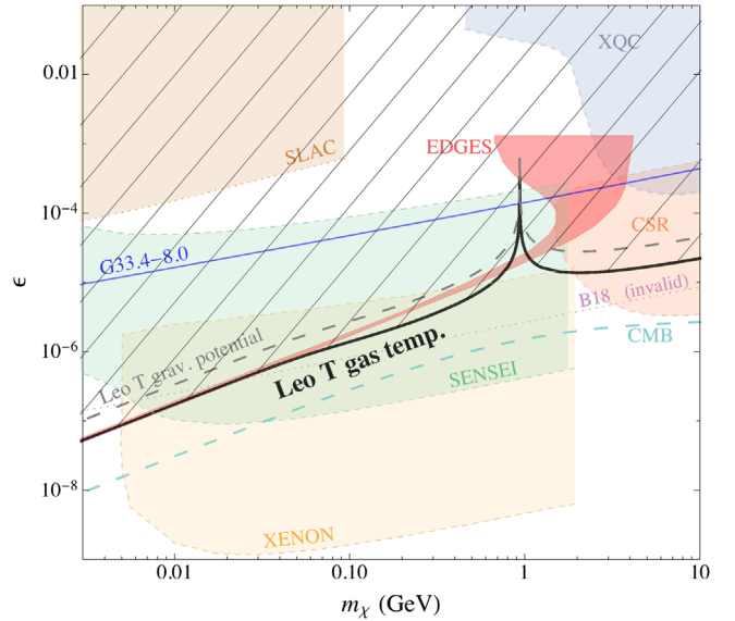
FIG. 3. Upper bound on the charge of DM from the Leo T galaxy (black); these constraints can be extrapolated to the left and right using \epsilon_{\max} \sim 10^{-4.7} (m/\text{GeV}) and \epsilon_{\max} \sim 10^{-5.2} \sqrt{(m/\text{GeV})} . The dashed gray line approximately shows the fundamental constraint of the very existence of the Leo T DM halo. The blue line shows the upper bound from the best MW corotating gas cloud, G33.4–8.0, while the (invalid) constraint reported by B18 is shown by the purple dotted line. We show in red the parameter range, which explains the EDGES 21 cm anomaly taken from Ref. [112] (see also Refs. [29,98,113]). Note that the Leo T bounds cannot be trivially extrapolated for the case where only a fraction of DM ( f_{\text{DM}} ) is charged; see the text for details and for the other constraints shown.
