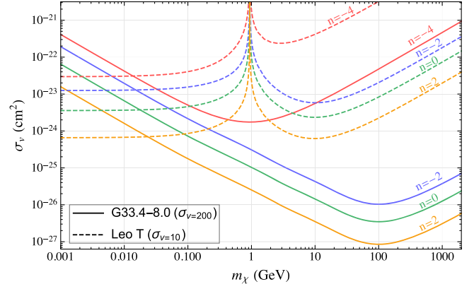
FIG. 4. Upper bounds on the DM-nucleon scattering cross section from the gas temperature of the cloud G33.4–8.0 (solid) and Leo T (dashed), for velocity dependence \sigma_{n\chi}(v) = \sigma_{v_0}(v/v_0)^n for n = 0, \pm 2, -4 . Note that the cross section limits are shown at different velocities—namely, the typical values constrained by the systems ( v_0 = 10 km/s for Leo T and v_0 = 200 km/s for the MW cloud). For n = -4 , the bound from Leo T for sub-GeV DM is comparable to the strongest bound in the current literature, which is from the CMB analysis by Ref. [28] (see Fig. 10).
