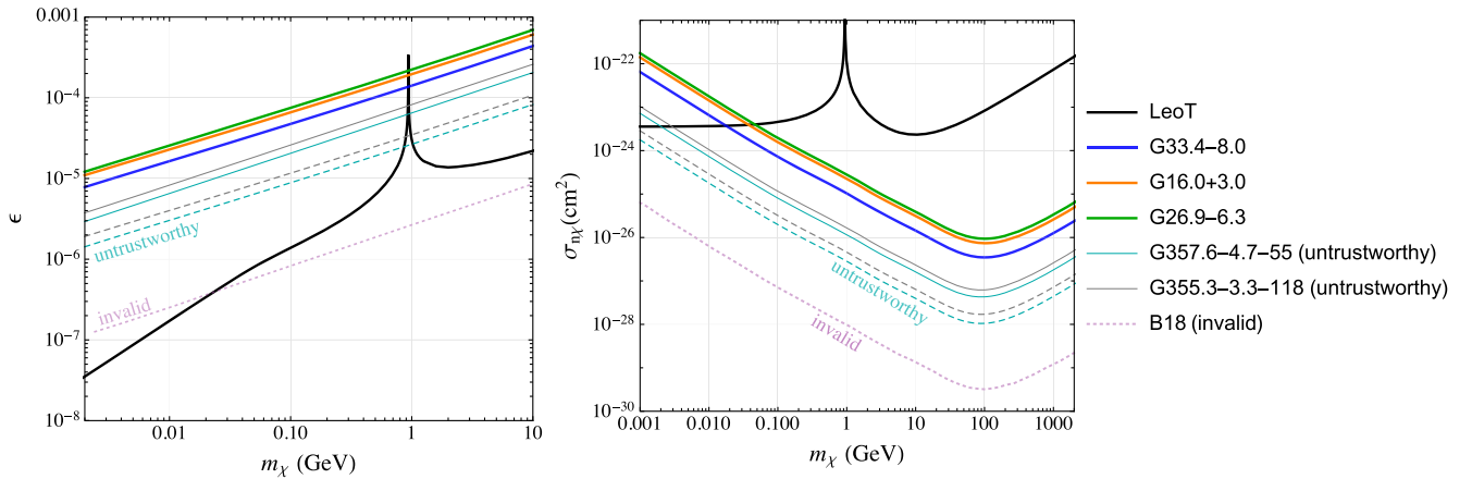
FIG. 5. Limits on \epsilon (left panel) and the DM-nucleon velocity-independent cross section \sigma_{n\chi} (right panel). The bound from Leo T is shown in black, and the bounds from the three best corotating MW gas clouds are shown as solid blue, orange, and green lines. The bounds from the two best Galactic high-velocity nuclear outflow clouds are shown as thin cyan and gray lines; the solid lines are the bounds when the best-fit Burkert profile from Ref. [138] is used for the DM halo, and the dashed lines are the bounds when the NFW profile from Ref. [139] is used. For the corotating clouds, the change in bounds when the Burkert profile is used instead of NFW is insignificant. The dotted line is the bound claimed by B18. Solar metallicity is assumed for all the clouds.
