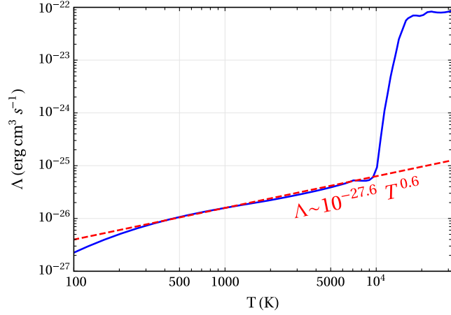
FIG. 7. The radiative cooling function from [90] for H I gas with solar metallicity (solid blue line). A convenient approximation for the cooling function \Lambda(T) = 10^{-27.6} T^{0.6} for T \sim (300\text{--}8000) K is shown as the dashed line.
