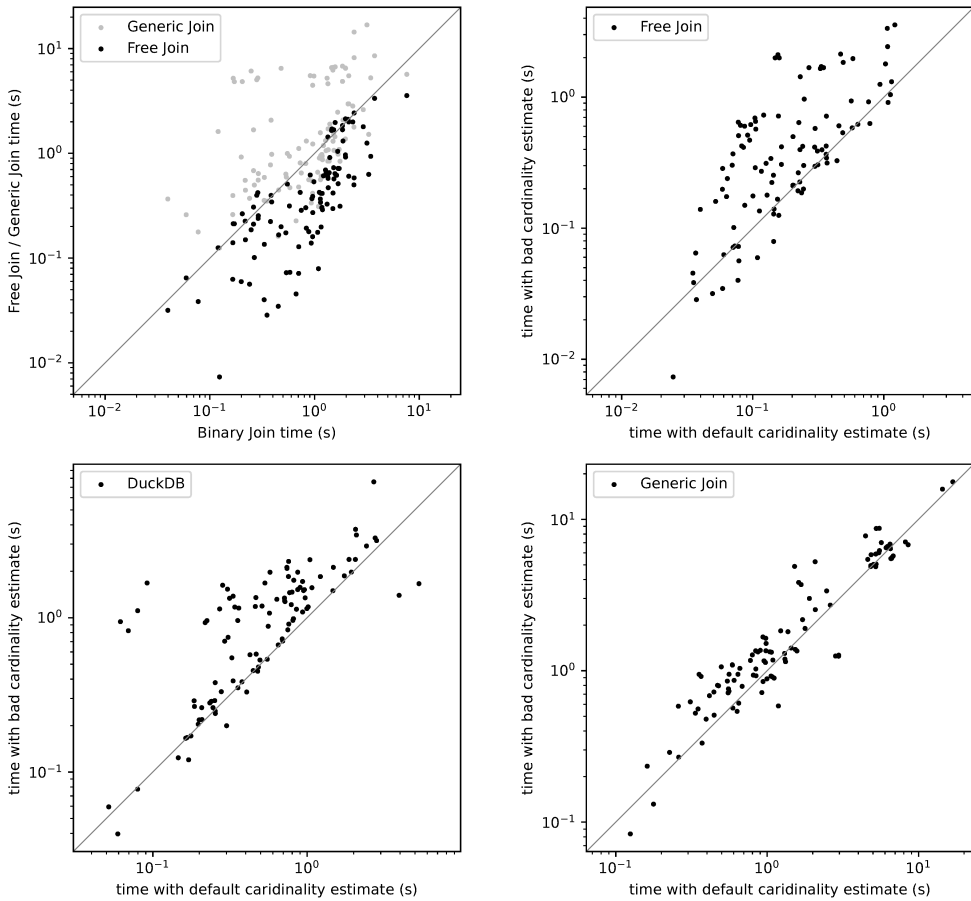
Fig. 18. Run time of join algorithms with good and bad cardinality estimates. The first plot compares the run time of Free Join, Generic Join and binary join on JOB with bad cardinality estimates. The remaining three plots compare the run time of each algorithm with good and bad cardinality estimates on JOB.
