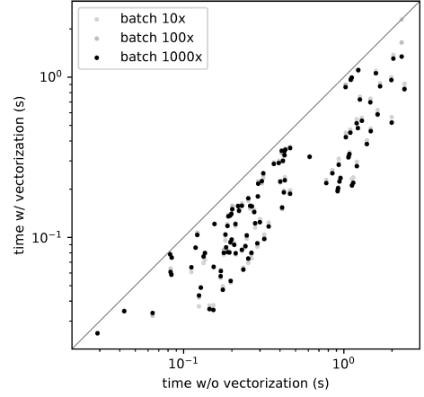
Fig. 17. Impact of vectorization.
