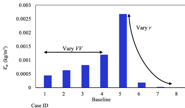
Fig. 5. Average concentrations in the wall region ( \overline{C_w} ) from Table 3 data.
