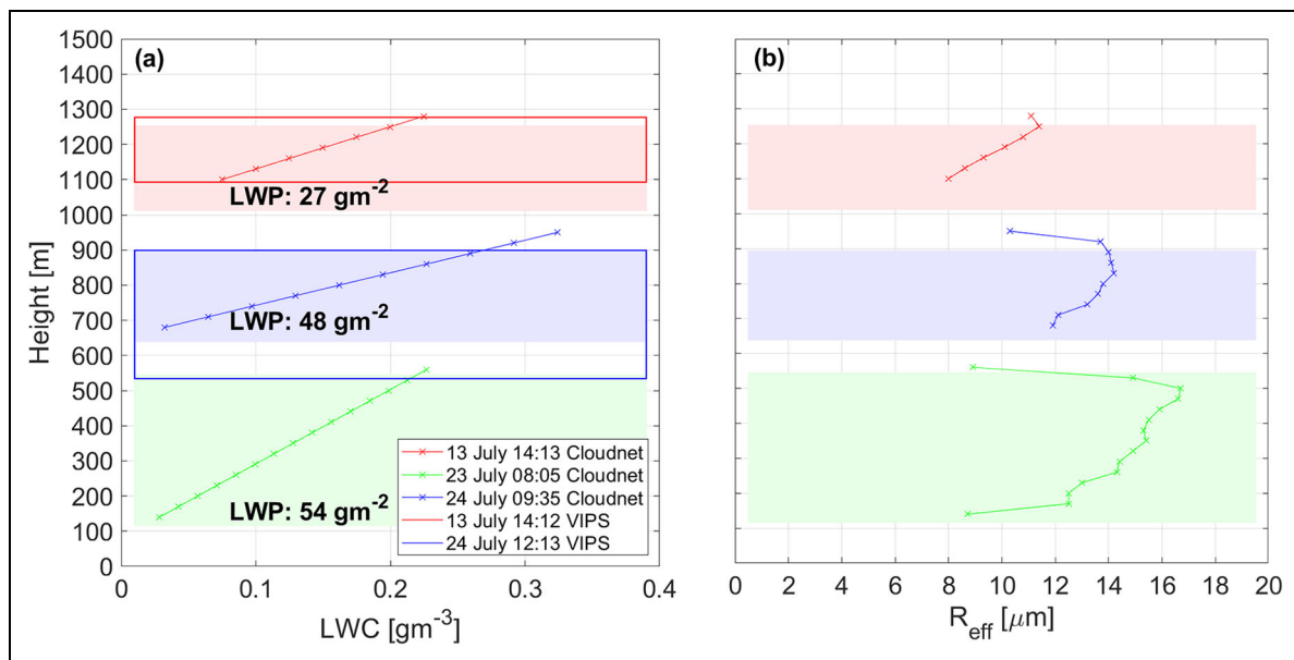
Figure 7. Cloud (a) liquid water content (LWC) and (b) particle effective radius R_{\text{eff}} . Profiles of (a) LWC and (b) particle effective radius ( R_{\text{eff}} ) derived from Cloudnet for July 13 (red), July 23 (green), and July 24, 2020 (blue). Shaded rectangles indicate the cloud cover derived from the broadband radiation package, and the empty rectangles the cloud cover indicated by Video Ice Particle Sampler (VIPS). Liquid water paths by Cloudnet are displayed as text. Note that VIPS data on July 24 are not from the same flight, while no VIPS data are available for July 23.
