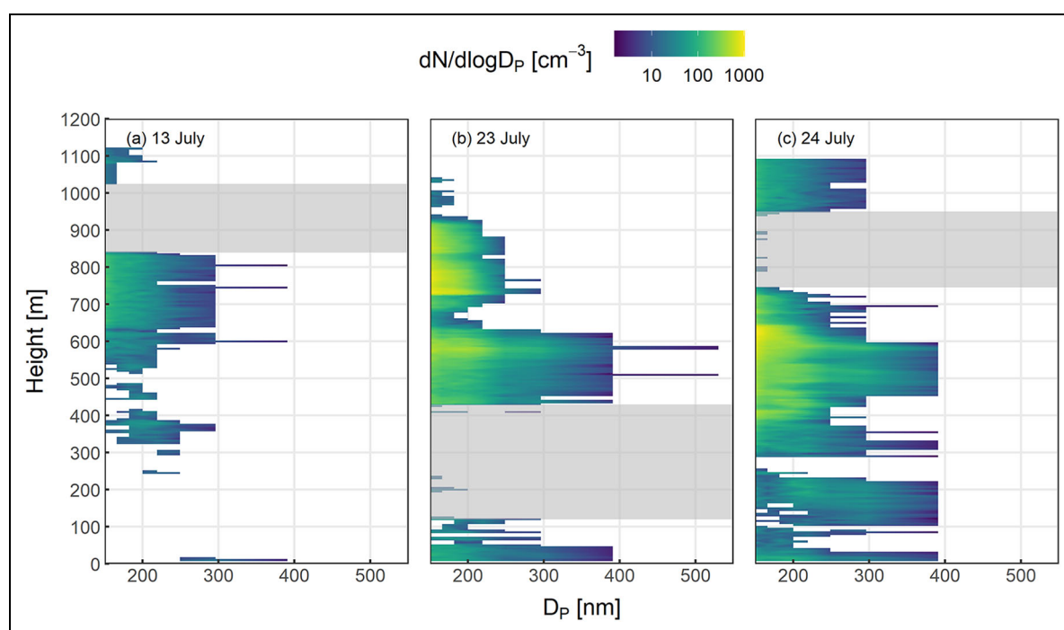
Figure 14. Profiles of particle number size distribution. Particle number size distributions were measured with an optical particle size spectrometer on (a) July 13, (b) July 23, and (c) July 24, 2020. A total of 14 bins covered a particle diameter range from 0.15 to 2.9 \mu\text{m} . Profiles are displayed as median distributions averaged over 5-m height steps. Gray shaded areas indicate the cloud cover derived from ship-based remote sensing in combination with BELUGA in situ observations. BELUGA = Balloon-borne moduLar Utility for profilinG the lower Atmosphere.
