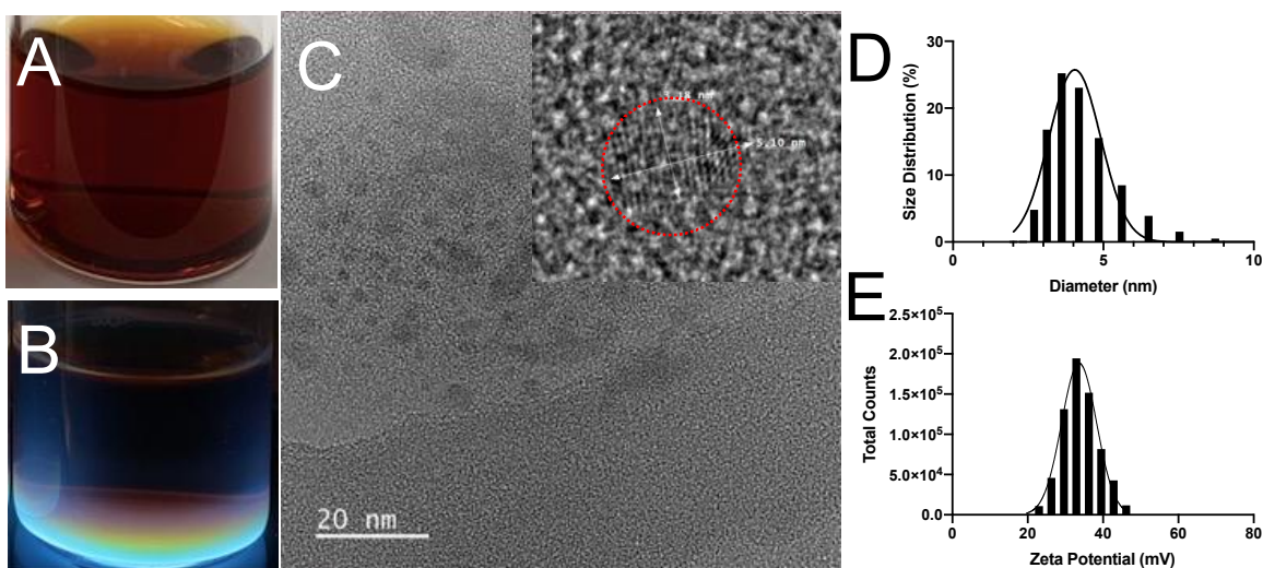
Figure 2. Characterization of the SiQD nanomaterials. (A) and (B) Photographs are shown of the SiQDs under white light and UV light illumination, respectively. (C) HR-TEM image of the SiQDs is shown with the scale bar of 20 nm. The inset panel is a magnified image with a clear lattice space of a SiQD. (D) The hydrodynamic diameter of the SiQDs was measured by DLS and graphed as a size distribution across the quantified population of SiQDs. (E) The zeta potential of the SiQDs was measured by DLS with the total counts graphed across the mV range assessed. The results shown are representative of 3 independent preparations with similar results.
