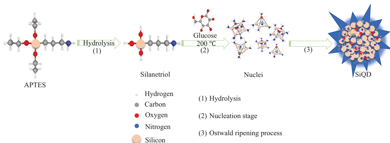
Figure 1. Schematic diagram of the synthetic process for SiQDs using glucose as the reducing agent. Step (1) APTES was first hydrolyzed to form aminopropyl silanetriol. Step (2) Aminopropyl silanetriol was transformed into unstable nuclei during the nucleation stage under 200 °C and in the presence of the reducing agent, glucose. Step (3) In the Ostwald ripening process, small, unstable nuclei were easily adsorbed and desorbed to form stable dots with luminescence capacity.
