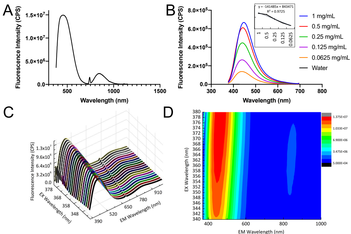
Figure 4. The fluorescence properties of potential dual-emissive SiQDs. (A) The emission spectrum of SiQDs is shown. (B) The emission spectra are compared for different concentrations of SiQDs, showing the emission peak at 447 nm. The inset graph is the calibration curve of different concentrations of SiQDs under emission of 447 nm. (C) The 3D spectra of SiQDs are
