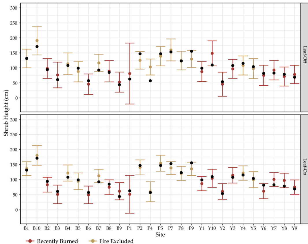
Figure 4. Mean shrub heights based on 40 ground samples (black dots) and predicted shrub heights obtained using multiple linear regression and TLS metrics calculated from leaf-off and leaf-on data. Error bars provide the 95% confidence PI for each plot.
