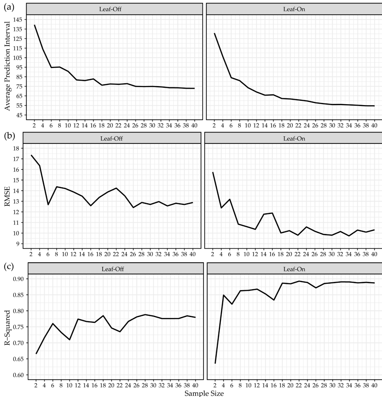
Figure 5. Changes in model performance with field reference data sample size. (a) Mean PI; (b) RMSE; (c) prediction R-squared.
