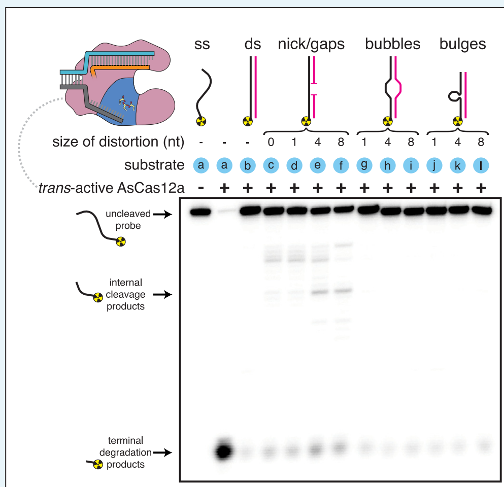
Appendix 1—figure 1. Substrate specificity of Cas12a trans -active holoenzyme. Phosphorimage of AsCas12a cleavage products, resolved by denaturing PAGE. Trans -active AsCas12a holoenzyme (115 nM of each component: protein, crRNA, pre-cleaved activator) was incubated with 1 nM of the indicated substrate for 2 hours at 30°C prior to quenching. Substrate (a) was a single-stranded DNA oligonucleotide with no homology to the crRNA. To generate substrates (b) through (l), substrate (a) was hybridized to a variety of unlabeled complementary DNA oligonucleotides. Substrate (c) contained a nick. Substrates (d), (e), and (f) contained gaps of 1, 4, and 8 nt, respectively. Substrates (g), (h), and (i) contained bubbles of 1, 4, and 8 nt, respectively. Substrates (j), (k), and (l) contained bulges of 1, 4, and 8 nt, respectively.
