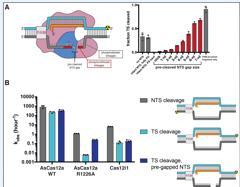
Appendix 2—figure 2. Non-target-strand gap formation poses a kinetic barrier to target-strand cleavage for AsCas12a. (A) Extent of target-strand cleavage by wild type AsCas12a in the presence of various non-target-strand variants, as resolved by denaturing PAGE (phosphorimage in Appendix 2—figure 2—figure supplement 5 ). Cas12a surveillance complex (100 nM AsCas12a, 120 nM crRNA) was added to 1 nM pre-hybridized target DNA radiolabeled on the 5' end of the TS and allowed to incubate in cleavage buffer with 5 mM \text{CaCl}_2 for 1 hr at 37°C prior to quenching. In the schematic, the red portion of the NTS denotes phosphorothioate (PS) linkages; the gray portion denotes phosphodiester (PO) linkages. In the graph, red bars denote reactions with a PS-containing NTS variant; gray bars denote reactions either with no NTS or with an NTS variant containing only PO-linkages. From left to right (omitting the no-NTS control), the NTS variants used were A, B, D, G, J, N, Q, T, W, Y, Z, as schematized in Appendix 2—figure 2—figure supplement 4 . Columns and associated error bars indicate the mean and standard deviation of three replicates. (B) Cleavage kinetics of NTS, TS, and TS complexed with a pre-gapped NTS (NTS contains a 5-nt gap). 100 nM protein and 120 nM cognate crRNA were incubated with 2 nM DNA target with a 5' radiolabel on the indicated strand at 37°C for various timepoints, followed by quenching and resolution by denaturing PAGE. Representative phosphorimages and quantifications are
