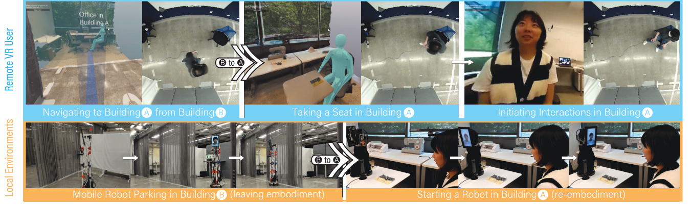
Figure 11: Demonstrations of switching between robotic proxies across multiple buildings. Using VRoxy, the VR user can navigate from the lab space in Building B to the office in Building A where the fixed robot is located to meet another collaborator. On the other side, the mobile robot in Building B starts parking to indicate the leave, and the stationary robot in Building A turns the body to face the collaborator to signify the re-embodiment.
