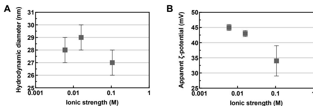
Figure 1. (A) Number-average hydrodynamic diameters and (B) \zeta -potential of poly(allylamine HCl)-wrapped diamond nanoparticles (PAH-DNPs) as a function of solution ionic strength. Solutions were buffered to pH 7.4 with 0.01 M Tris and ionic strength adjusted with NaCl. Data points represent the mean of six replicates. Error bars denote one standard deviation. Numerical data are tabulated in Table S2.
