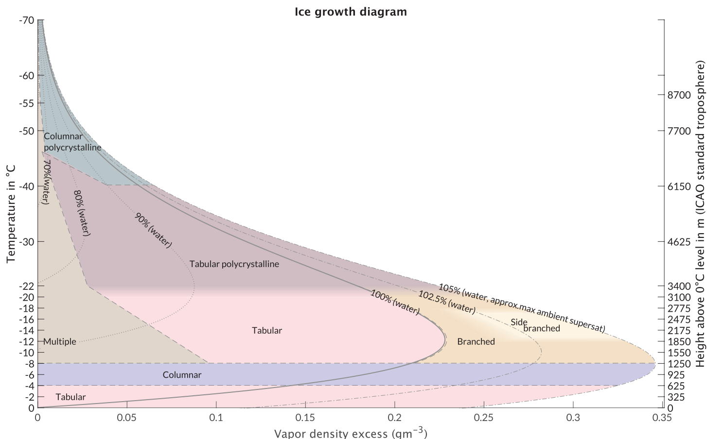
Fig. 3. Ice growth forms diagram in terms of vapor density excess over ice saturation with contours of RH_w overlaid. The ICAO approximation on the right y axis is offset by the height of the 0°C level. T_{ice} = T_{air} is assumed (St-Pierre and Thériault 2015). Dashed lines indicate uncertainty in the exact bounding conditions between different ice growth forms. Blurred regions indicate transition zones between ice growth forms.
