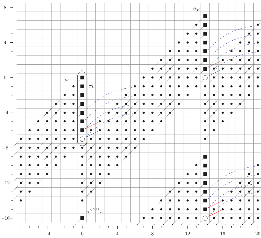
FIGURE 1. The slice E_\infty term for k_{GL}(3) , together with extensions. See Remark 3.6 for the notation.
