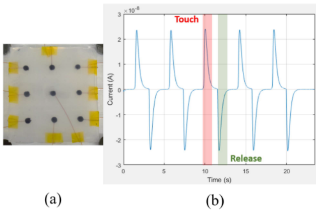
Fig. 6. (a) TENG device (size at around 5 cm \times 5 cm). (b) Electrical output of TENG under periodic physical contacts (sampled at 1000 Hz).
