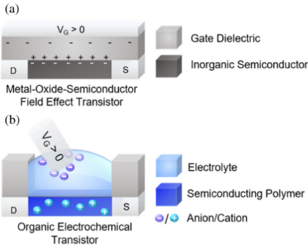
Fig. 1. Comparison of the device structure of (a) metal-oxide-semiconductor field effect transistor and (b) organic electrochemical transistor (OECT).
