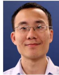
ificial intelligence.
