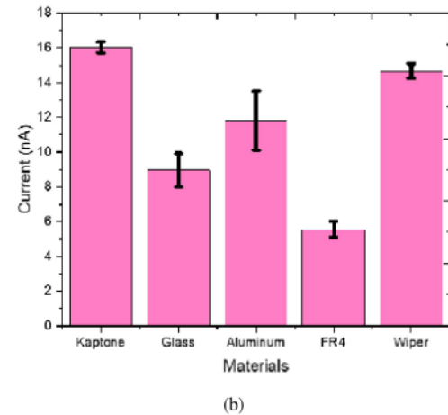
Fig. 9. (a) Relationship between the TENG electrical output and input pressure (red line: linear regression result). (b) Different TENG electrical output amplitude for various contact materials.
