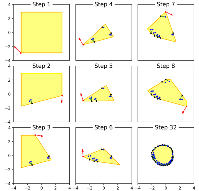
Fig. 2. Steps of the construction of a polyhedral Lyapunov function for the system of Example 3, with \epsilon = 3 , \tau = 1/4 and \gamma = 1 . At each step k = 1, \dots, 32 , a polyhedral function V_k (yellow region), satisfying the conditions of Proposition 13 at the witness set X_k (black dots), is computed. Then, the algorithm checks whether it can find a counterexample x_k (red dots). After 32 steps, the process has computed a polyhedral Lyapunov function for the system (last plot). (For interpretation of the references to color in this figure legend, the reader is referred to the web version of this article.)
