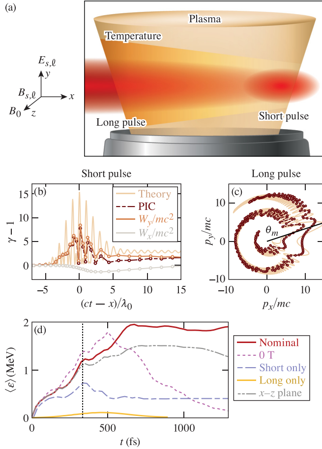
FIG. 1. Generation of relativistic underdense plasma via magnetically assisted direct laser acceleration. (a) Illustration of laser and magnetic-field configuration. [(b), (c)] Example of the energy gain process for a representative electron interacting with (b) the short pulse, and (c) the long pulse. W_y ( W_x ) is the work done by the transverse (longitudinal) electric field. (d) Average energy of all electrons in r < 25 \mu\text{m} . Black dotted line: the time the peak of the short pulse leaves the plasma slab. At the final time shown, the long pulse intensity has dropped to a_\ell/e at the right edge of the slab. The nominal case corresponds to both laser pulses and B_{z0} = 500 \text{ T} , simulated in the x - y plane.
