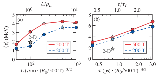
FIG. 4. Strategies for improving average electron energy in 1D PIC simulations. (a) Scan over plasma size near L/\rho_L \sim 1 with fixed duration. (b) Scan over long-pulse duration near \tau_\ell/\tau_L \sim 1 with fixed plasma size. \rho_L and \tau_L are the Larmor radius and cyclotron period associated with \Delta\gamma . The starred points are shared between (a) and (b). The peak of the short pulse is kept coincident with a_\ell/e on the rising edge of the long pulse. \tau_s = 50 fs for the 200-T cases.
