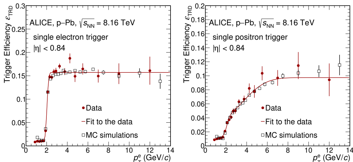
Figure 1. Acceptance times efficiency of the TRD trigger with the p_T threshold at 2 GeV/c for single electrons (left) and single positrons (right) obtained from data and MC simulations. See text for details.
