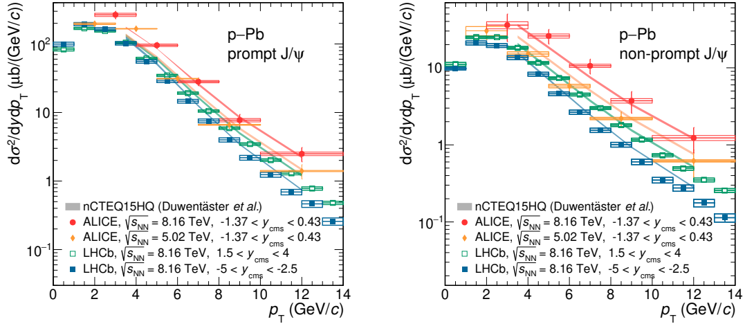
Figure 8. p_T -differential production cross sections of prompt (left) and non-prompt (right) J/\psi together with corresponding results at forward and backward rapidity by the LHCb collaboration [22] and ALICE measurements at midrapidity at \sqrt{s_{NN}} = 5.02 TeV [20]. The statistical and systematic uncertainties are represented as error bars and boxes for each data point. The normalisation uncertainties are not shown. The measurements are compared with calculations using the latest version of the CTEQ nPDFs, nCTEQ15HQ [80], see text for details.
