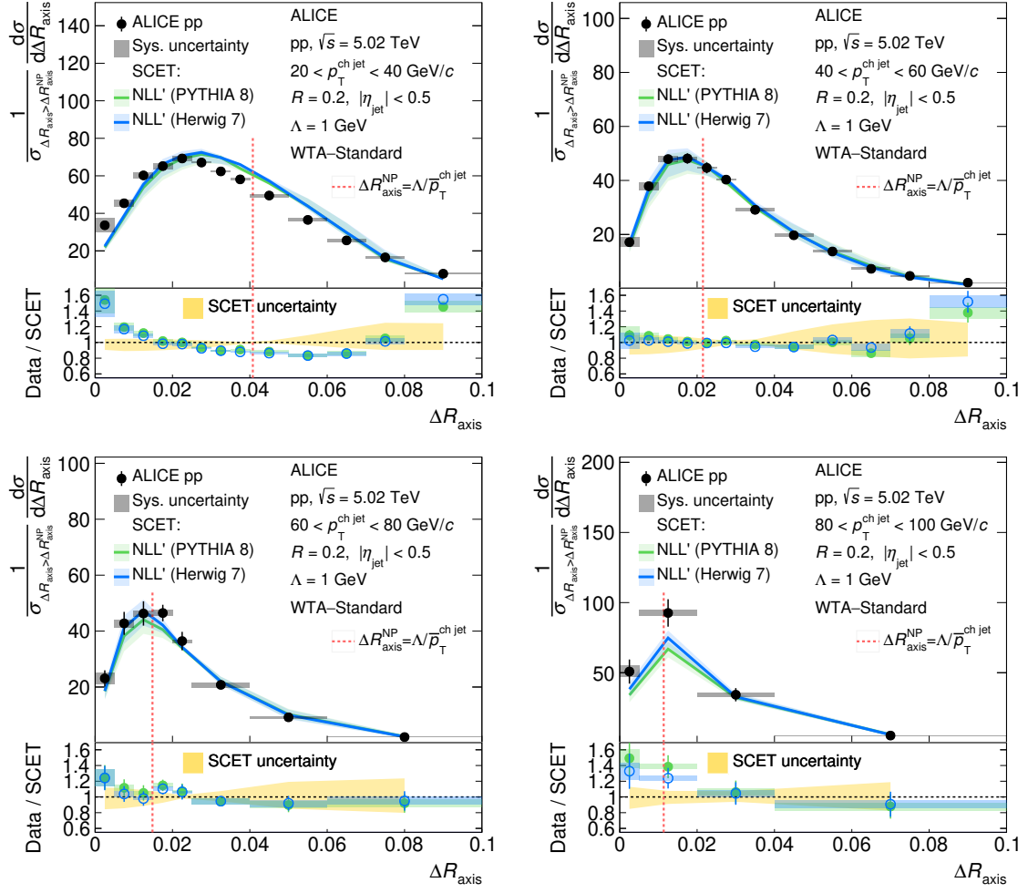
Figure 25. Same as figure 18, for WTA-Standard for R = 0.2 .
