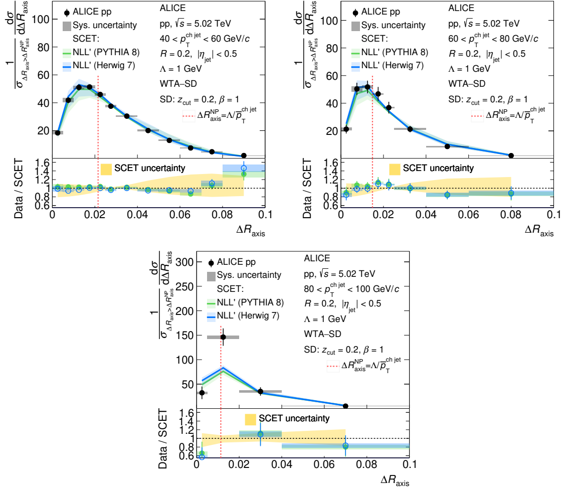
Figure 30. Same as figure 18, for WTA-SD ( z_{\text{cut}} = 0.2 , \beta = 1 ) for R = 0.2 .
