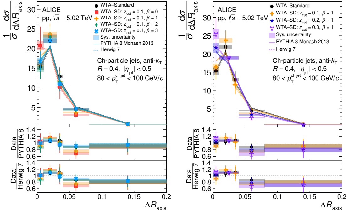
Figure 10. Same as figure 6 for 80 < p_T^{\text{jet}} < 100 GeV/c.
