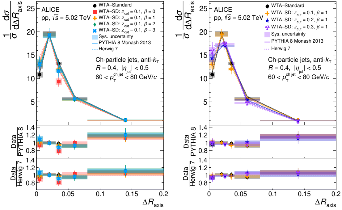
Figure 8. Same as figure 6 for 60 < p_T^{\text{jet}} < 80 \text{ GeV}/c .
