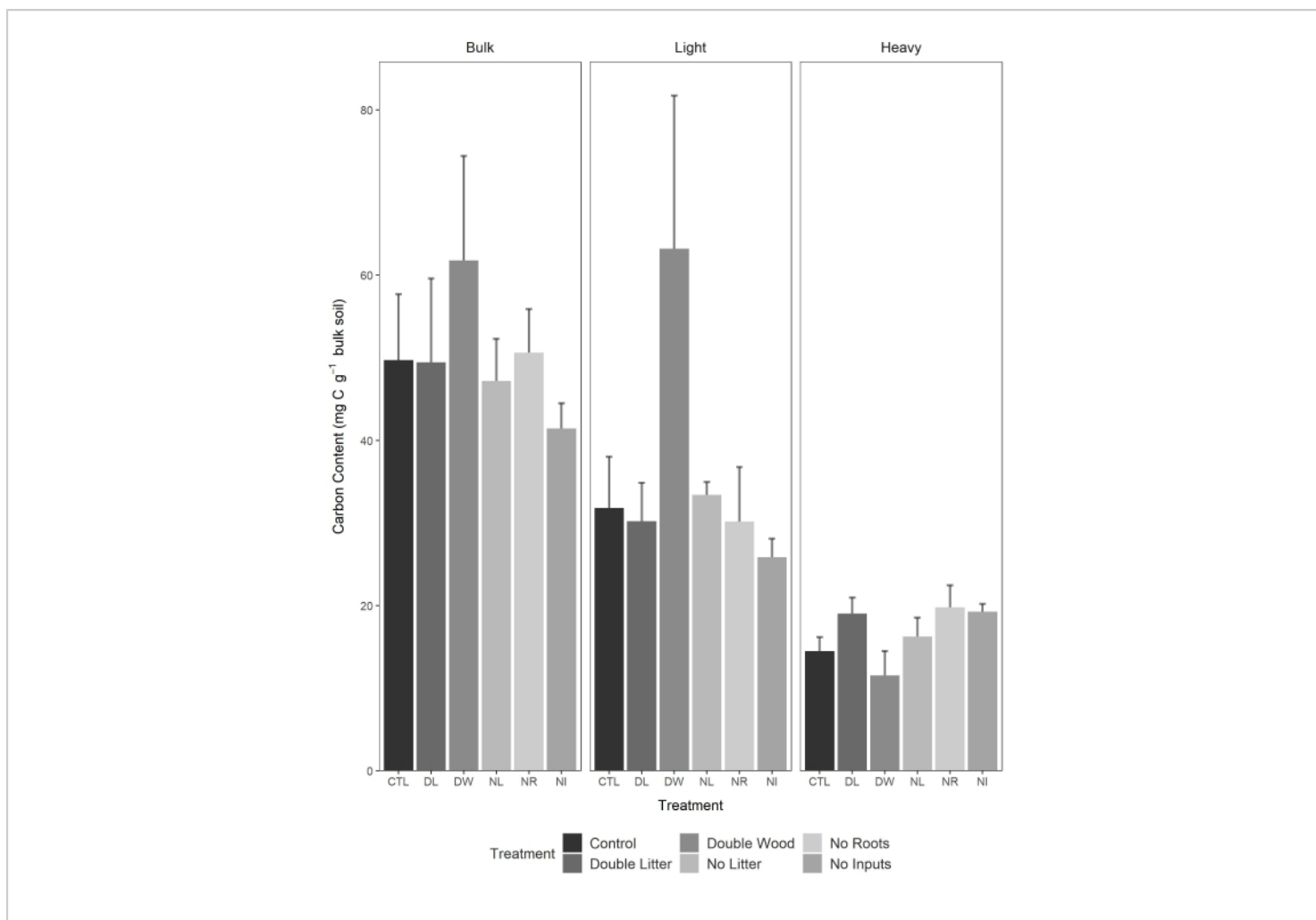
Figure 2: Comparison of the carbon content for bulk, light, and heavy fraction soil. Soil was collected from the Detrital Input and Removal Treatment (DIRT) plots in the H.J. Andrews Experimental Forest after 20 years of treatment ( n = 3 ). The mineral-associated C for the root removal treatments (NR, NI) was significantly increased, contrasting with the observed effects on bulk C content. Further, the fractionated results show that the increase in bulk C from the double wood (DW) treatment was derived from an increase in the light fraction C. The error bars represent the standard error. This figure has been modified from Pierson et al. 33 . Please click here to view a larger version of this figure.
