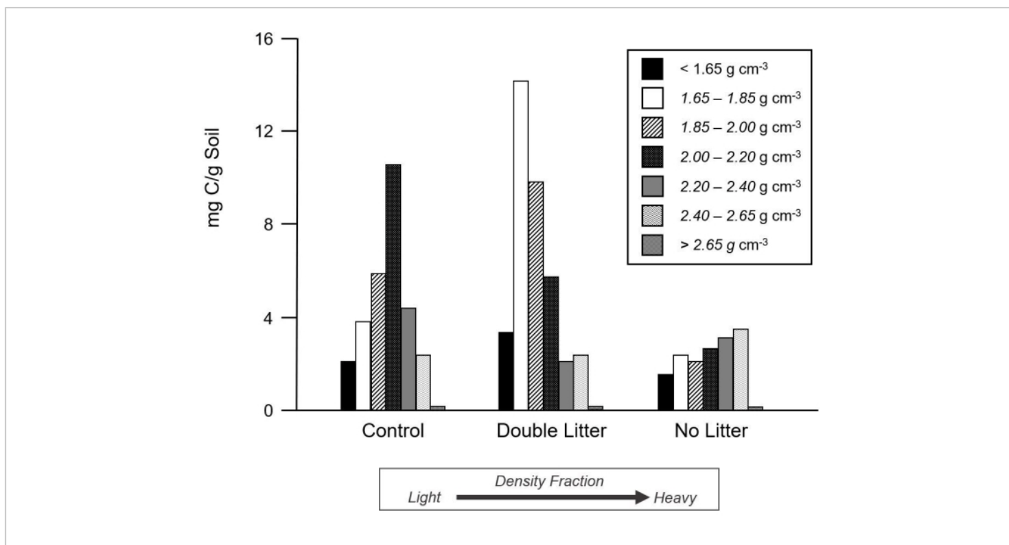
Figure 5: Sequential density fractionation of soil following 50 years of detrital manipulations (n = 4). Separating the soil into seven density fractions provided insight into the nature of the C loading on soil minerals. The double litter treatment, which increased soil C, led to the C loading of mineral material in the 2.00-2.40 g/cm 3 fraction, as shown by the change in the fraction C concentrations relative to the control. The losses of soil C from the no litter treatment were greatest in the soil fractions with densities between 1.85-2.20 g/cm 3 . The error bars represent the standard error. This figure has been modified from Lajtha et al. 22 . Please click here to view a larger version of this figure.
