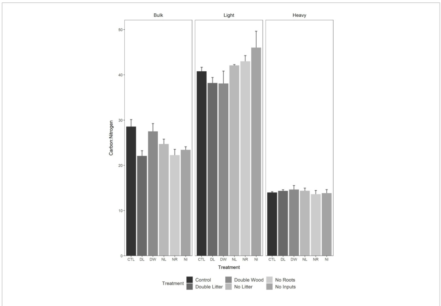
Figure 4: Carbon to nitrogen ratios for bulk, light, and heavy fraction soil. Soil was collected from the Detrital Input and Removal Treatment (DIRT) plots in the H.J. Andrews Experimental Forest after 20 years of treatment ( n = 3 ). Given the high C:N content of plant tissue relative to soil minerals, the observed difference in C:N content between the light and heavy fractions clearly demonstrates the capability of soil density fractionation to separate particulate organic matter from bulk soil. The error bars represent the standard error. This figure has been modified from Pierson et al. 33 . Please click here to view a larger version of this figure.
