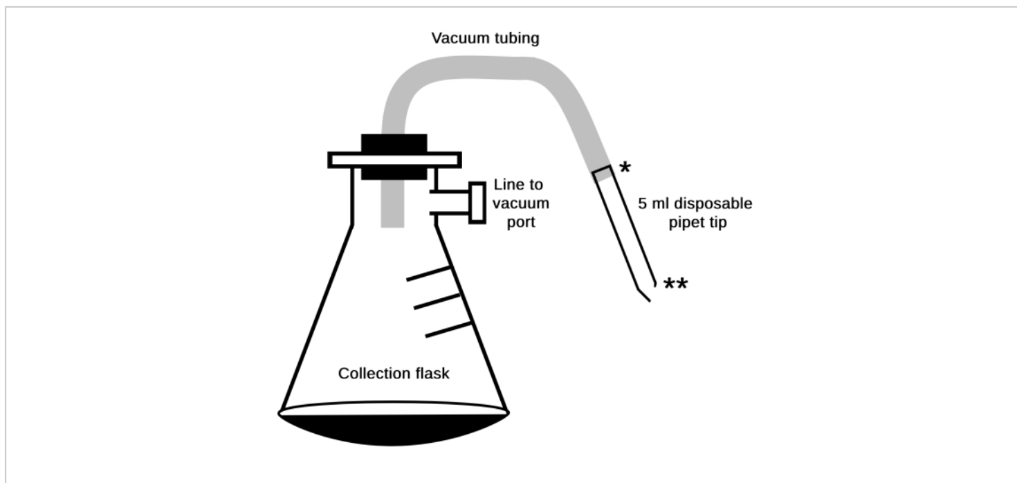
Figure 1: Light fraction aspiration apparatus. Schematic of the vacuum apparatus for the aspiration of the light fraction.
