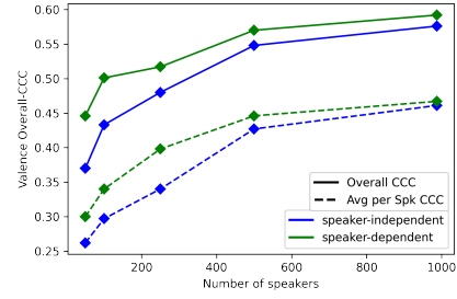
Figure 1: Performance gap between speaker-dependent and speaker-independent models for valence estimation with varying the number of training speakers.
